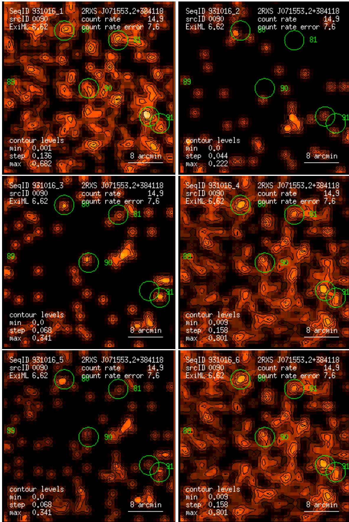
Figure 90: RASS 931016: detection 0090: band rate images, Gaussian filter: (1) PSPC channels 11 – 41, (2) 52 – 90, (3) 91 – 201, (4) 11 – 235, (5) 52 – 201, (6) 11 – 201. Broad band rates in counts/ks. Band rate contour levels in counts/ks/arcmin 2 .
