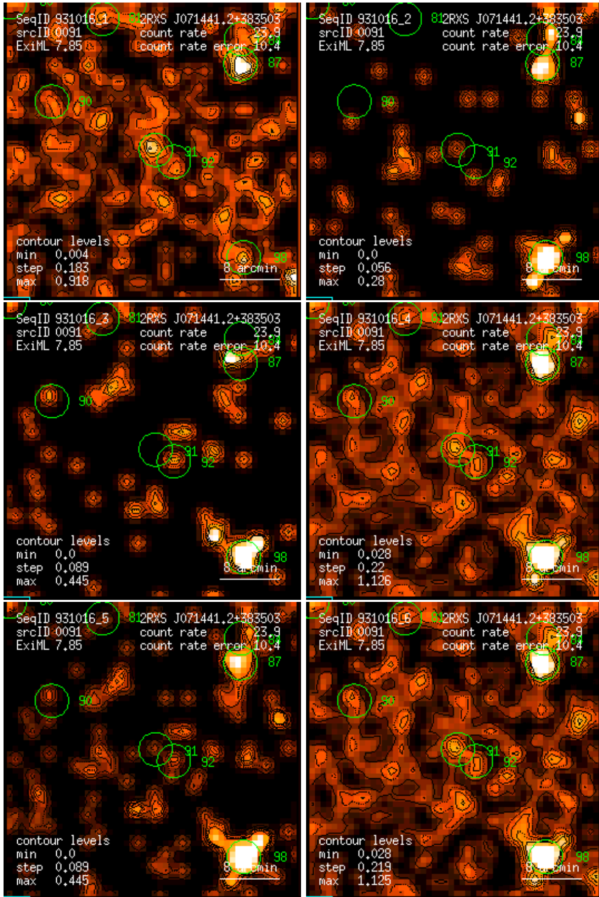
Figure 91: RASS 931016: detection 0091: band rate images, Gaussian filter: (1) PSPC channels 11 – 41, (2) 52 – 90, (3) 91 – 201, (4) 11 – 235, (5) 52 – 201, (6) 11 – 201. Broad band rates in counts/ks. Band rate contour levels in counts/ks/arcmin 2 .
