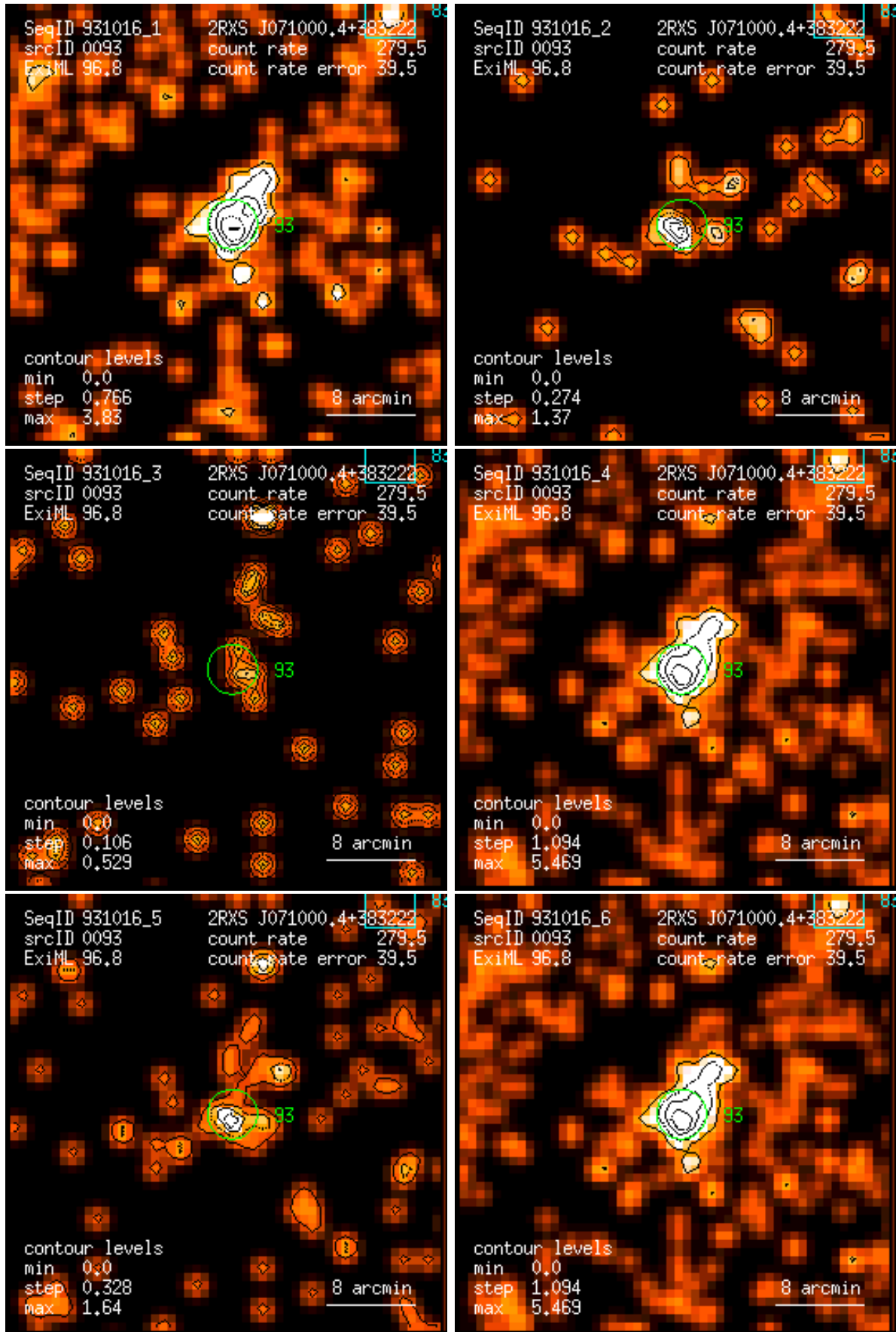
Figure 93: RASS 931016: detection 0093: band rate images, Gaussian filter: (1) PSPC channels 11 – 41, (2) 52 – 90, (3) 91 – 201, (4) 11 – 235, (5) 52 – 201, (6) 11 – 201. Broad band rates in counts/ks. Band rate contour levels in counts/ks/arcmin 2 .
