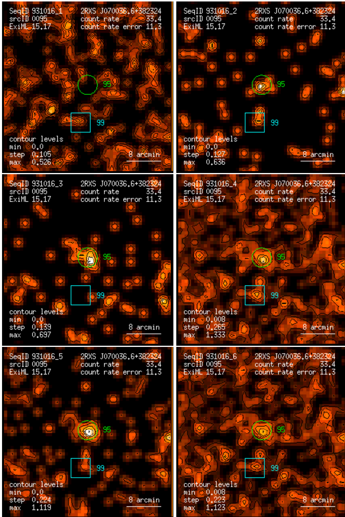
Figure 95: RASS 931016: detection 0095: band rate images, Gaussian filter: (1) PSPC channels 11 – 41, (2) 52 – 90, (3) 91 – 201, (4) 11 – 235, (5) 52 – 201, (6) 11 – 201. Broad band rates in counts/ks. Band rate contour levels in counts/ks/arcmin 2 .
