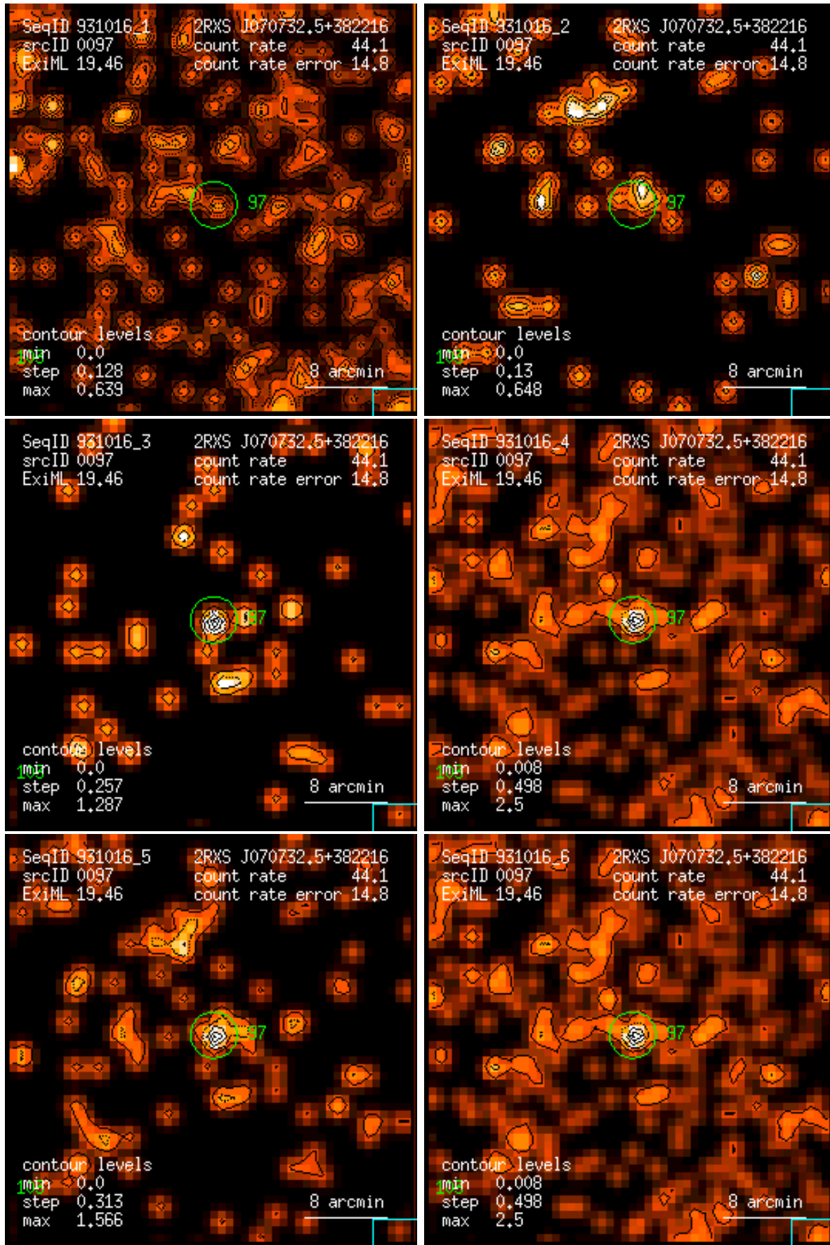
Figure 97: RASS 931016: detection 0097: band rate images, Gaussian filter: (1) PSPC channels 11 – 41, (2) 52 – 90, (3) 91 – 201, (4) 11 – 235, (5) 52 – 201, (6) 11 – 201. Broad band rates in counts/ks. Band rate contour levels in counts/ks/arcmin 2 .
