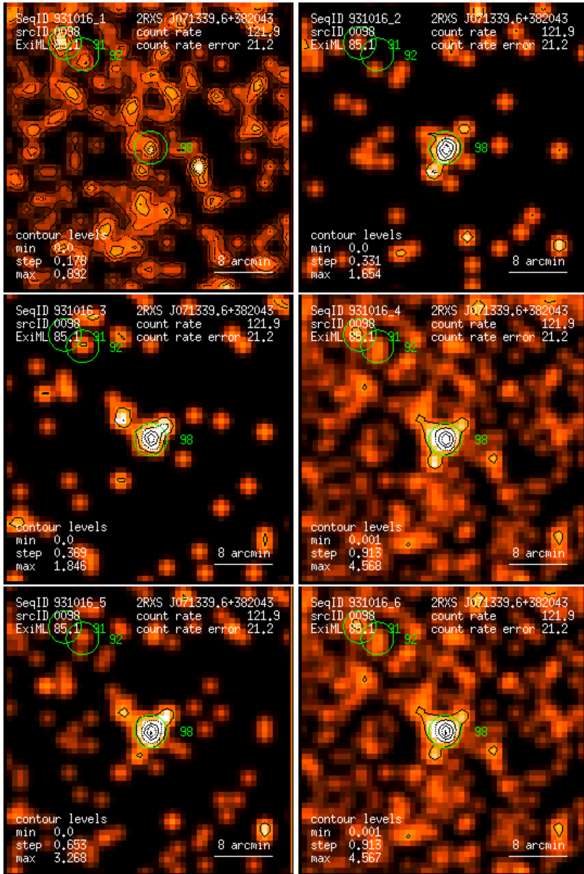
Figure 98: RASS 931016: detection 0098: band rate images, Gaussian filter: (1) PSPC channels 11 – 41, (2) 52 – 90, (3) 91 – 201, (4) 11 – 235, (5) 52 – 201, (6) 11 – 201. Broad band rates in counts/ks. Band rate contour levels in counts/ks/arcmin 2 .
