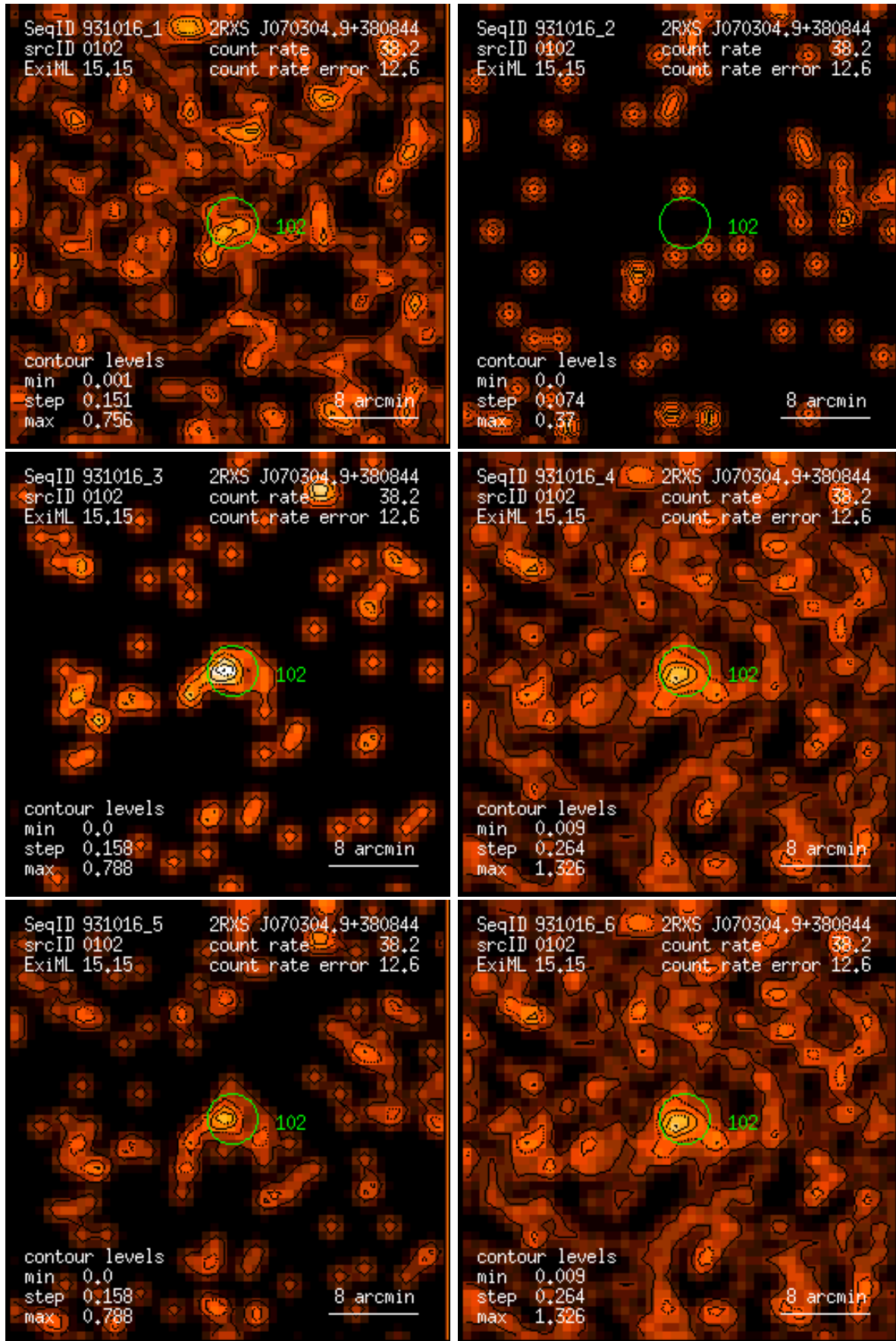
Figure 102: RASS 931016: detection 0102: band rate images, Gaussian filter: (1) PSPC channels 11 – 41, (2) 52 – 90, (3) 91 – 201, (4) 11 – 235, (5) 52 – 201, (6) 11 – 201. Broad band rates in counts/ks. Band rate contour levels in counts/ks/arcmin 2 .
