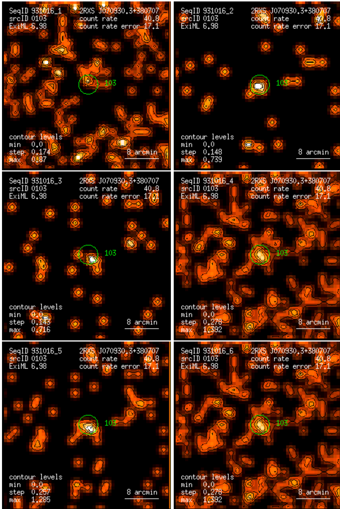
Figure 103: RASS 931016: detection 0103: band rate images, Gaussian filter: (1) PSPC channels 11 – 41, (2) 52 – 90, (3) 91 – 201, (4) 11 – 235, (5) 52 – 201, (6) 11 – 201. Broad band rates in counts/ks. Band rate contour levels in counts/ks/arcmin 2 .
