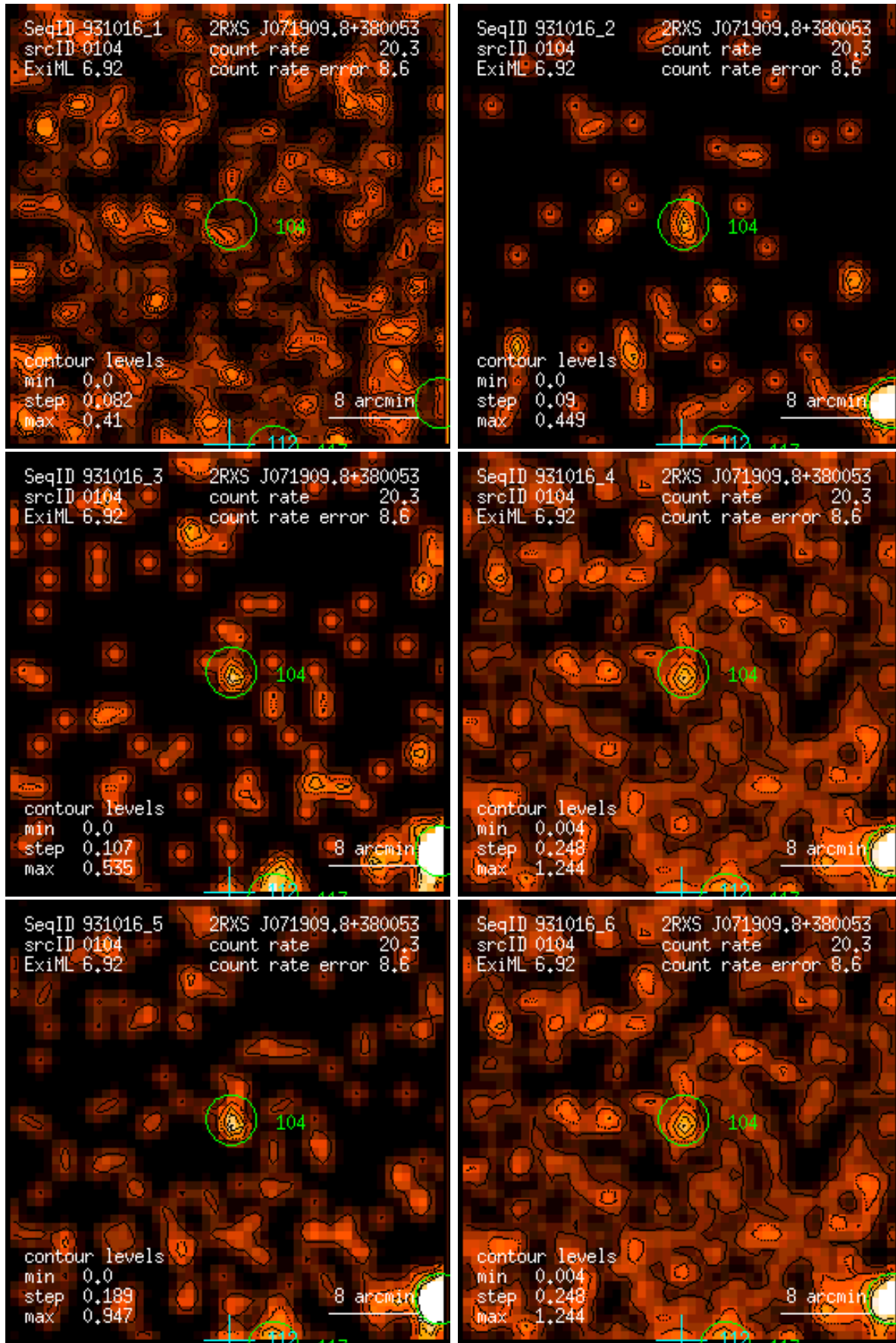
Figure 104: RASS 931016: detection 0104: band rate images, Gaussian filter: (1) PSPC channels 11 – 41, (2) 52 – 90, (3) 91 – 201, (4) 11 – 235, (5) 52 – 201, (6) 11 – 201. Broad band rates in counts/ks. Band rate contour levels in counts/ks/arcmin 2 .
