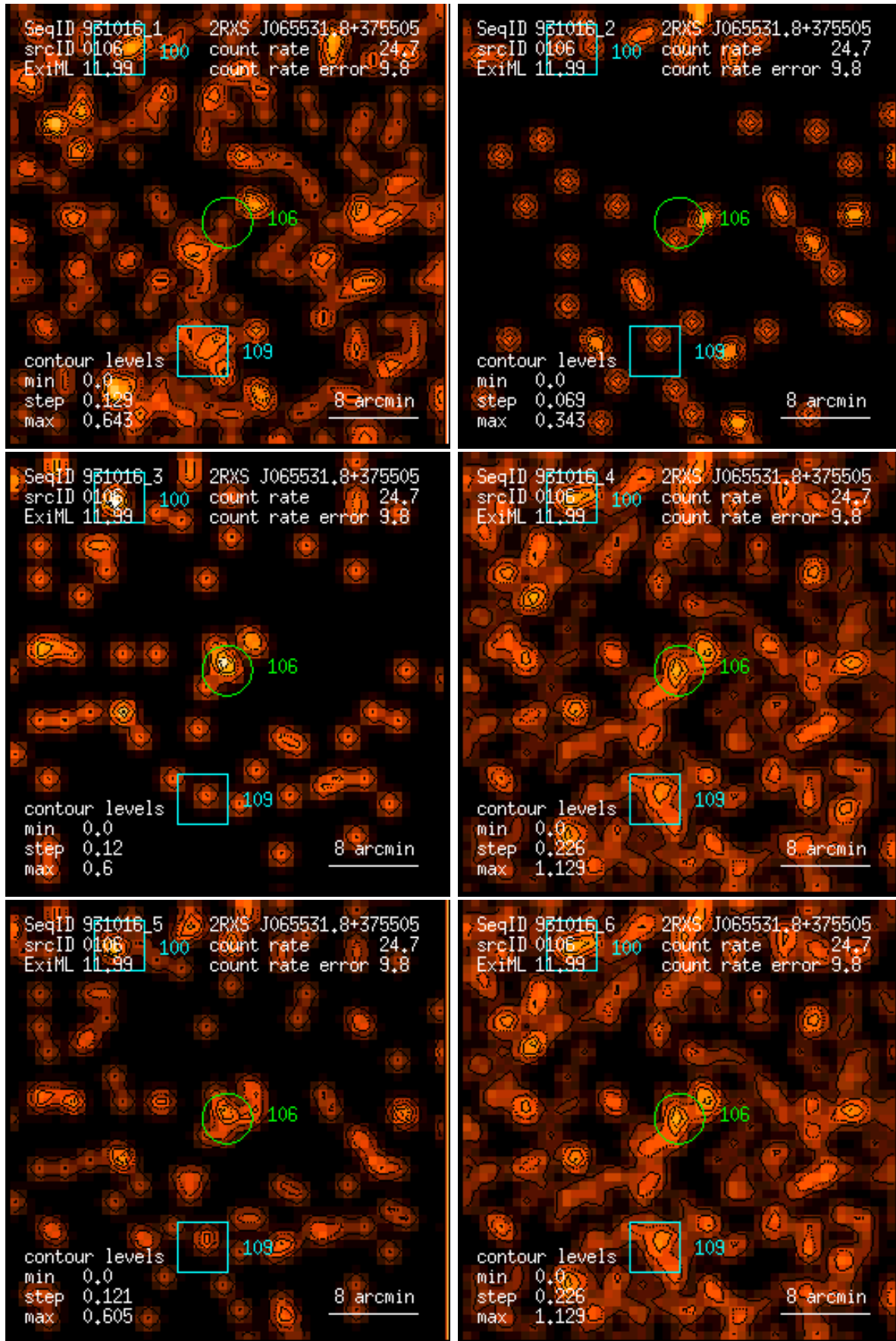
Figure 106: RASS 931016: detection 0106: band rate images, Gaussian filter: (1) PSPC channels 11 – 41, (2) 52 – 90, (3) 91 – 201, (4) 11 – 235, (5) 52 – 201, (6) 11 – 201. Broad band rates in counts/ks. Band rate contour levels in counts/ks/arcmin 2 .
