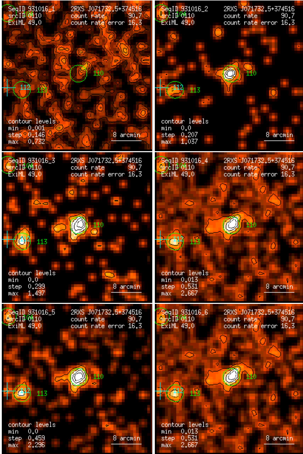
Figure 110: RASS 931016: detection 0110: band rate images, Gaussian filter: (1) PSPC channels 11 – 41, (2) 52 – 90, (3) 91 – 201, (4) 11 – 235, (5) 52 – 201, (6) 11 – 201. Broad band rates in counts/ks. Band rate contour levels in counts/ks/arcmin 2 .
