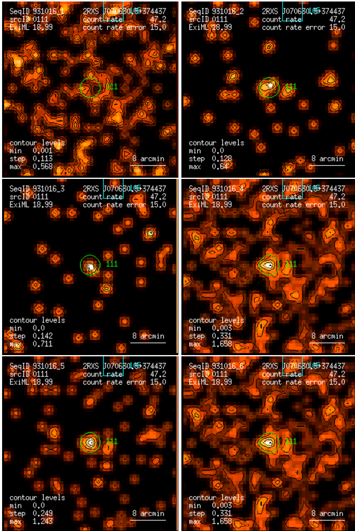
Figure 111: RASS 931016: detection 0111: band rate images, Gaussian filter: (1) PSPC channels 11 – 41, (2) 52 – 90, (3) 91 – 201, (4) 11 – 235, (5) 52 – 201, (6) 11 – 201. Broad band rates in counts/ks. Band rate contour levels in counts/ks/arcmin 2 .
