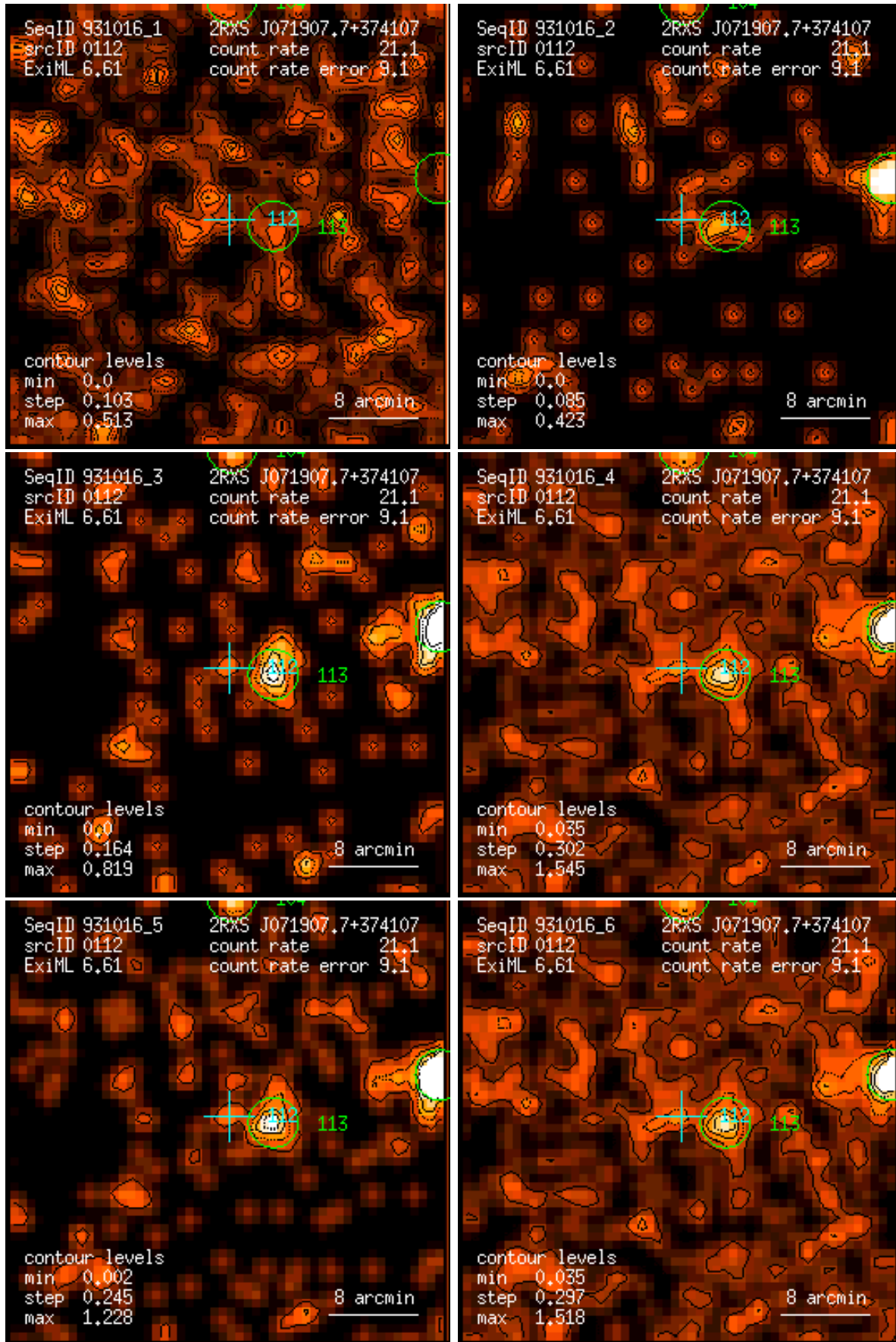
Figure 112: RASS 931016: detection 0112: band rate images, Gaussian filter: (1) PSPC channels 11 – 41, (2) 52 – 90, (3) 91 – 201, (4) 11 – 235, (5) 52 – 201, (6) 11 – 201. Broad band rates in counts/ks. Band rate contour levels in counts/ks/arcmin 2 .
