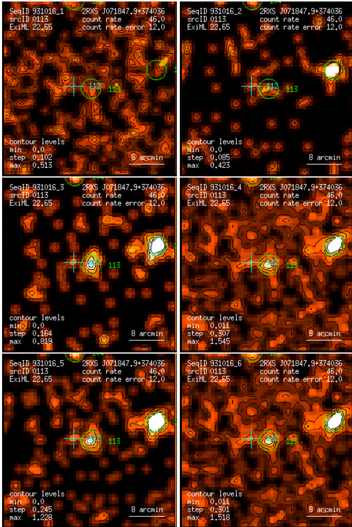
Figure 113: RASS 931016: detection 0113: band rate images, Gaussian filter: (1) PSPC channels 11 – 41, (2) 52 – 90, (3) 91 – 201, (4) 11 – 235, (5) 52 – 201, (6) 11 – 201. Broad band rates in counts/ks. Band rate contour levels in counts/ks/arcmin 2 .
