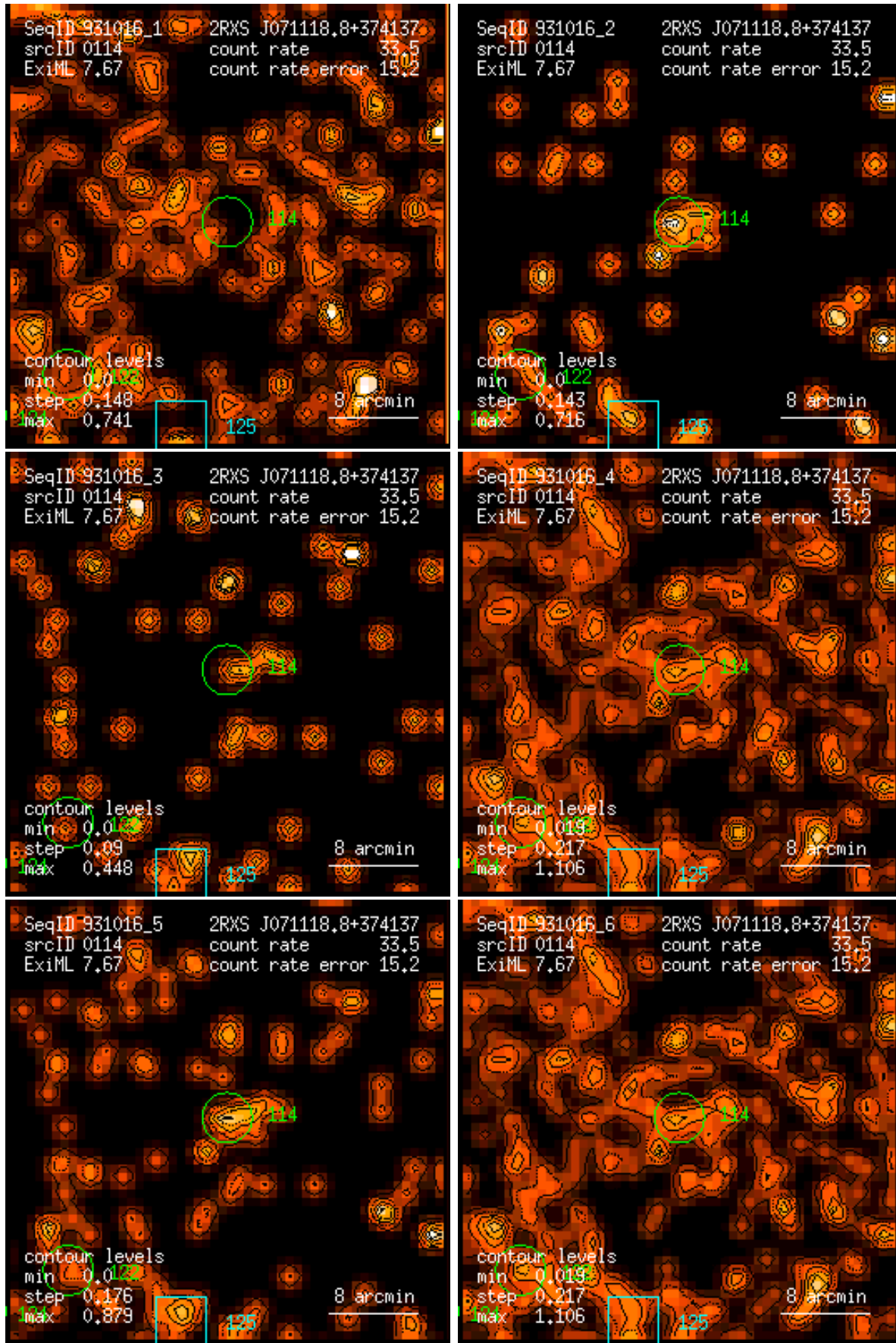
Figure 114: RASS 931016: detection 0114: band rate images, Gaussian filter: (1) PSPC channels 11 – 41, (2) 52 – 90, (3) 91 – 201, (4) 11 – 235, (5) 52 – 201, (6) 11 – 201. Broad band rates in counts/ks. Band rate contour levels in counts/ks/arcmin 2 .
