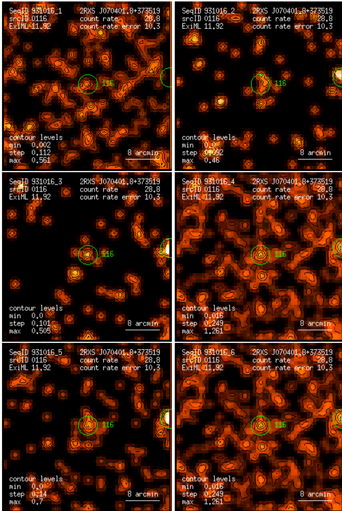
Figure 116: RASS 931016: detection 0116: band rate images, Gaussian filter: (1) PSPC channels 11 – 41, (2) 52 – 90, (3) 91 – 201, (4) 11 – 235, (5) 52 – 201, (6) 11 – 201. Broad band rates in counts/ks. Band rate contour levels in counts/ks/arcmin 2 .
