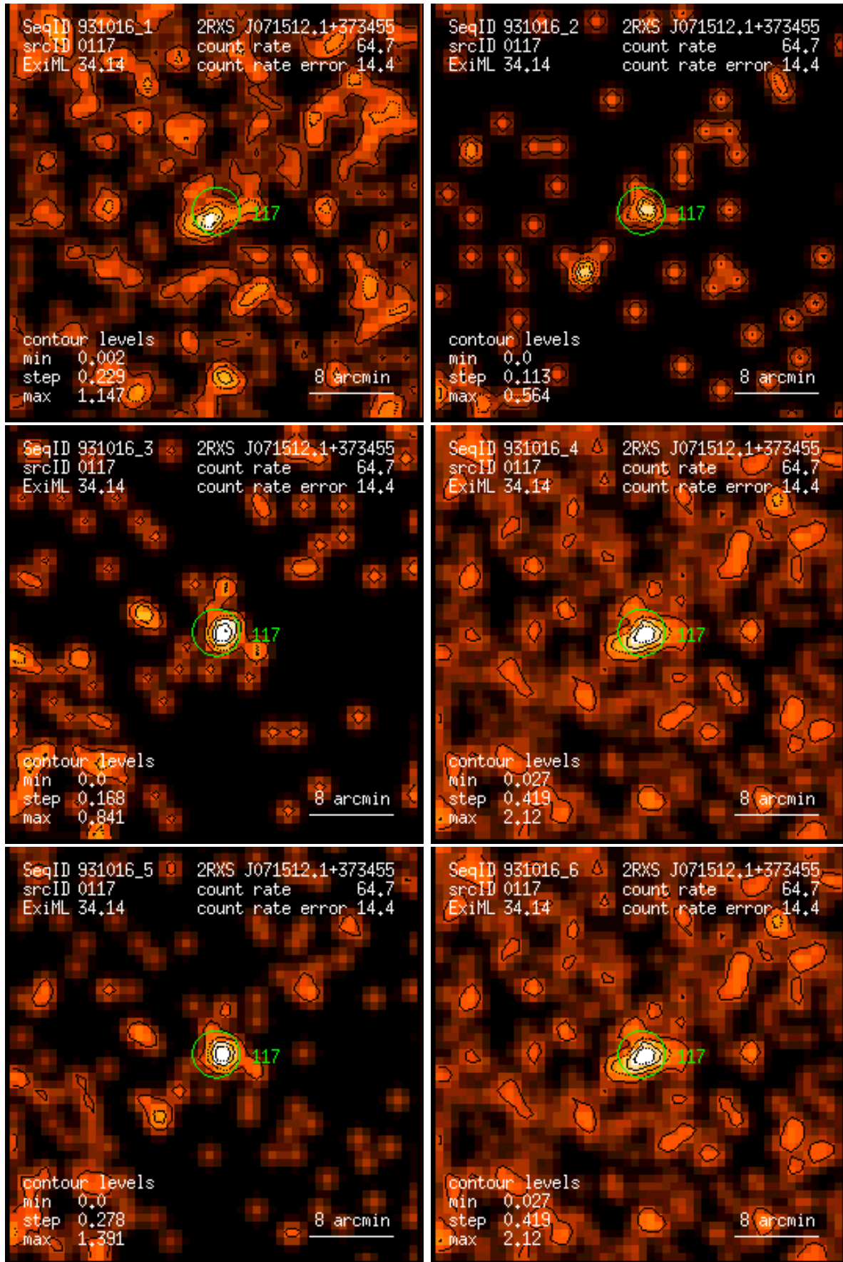
Figure 117: RASS 931016: detection 0117: band rate images, Gaussian filter: (1) PSPC channels 11 – 41, (2) 52 – 90, (3) 91 – 201, (4) 11 – 235, (5) 52 – 201, (6) 11 – 201. Broad band rates in counts/ks. Band rate contour levels in counts/ks/arcmin 2 .
