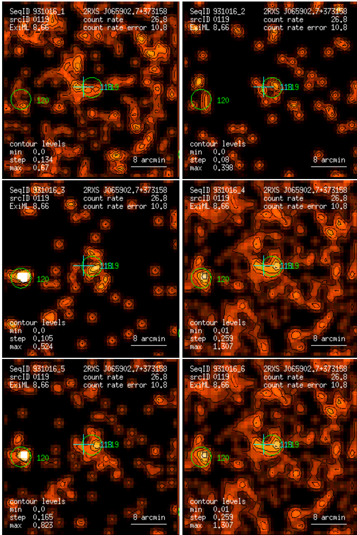
Figure 119: RASS 931016: detection 0119: band rate images, Gaussian filter: (1) PSPC channels 11 – 41, (2) 52 – 90, (3) 91 – 201, (4) 11 – 235, (5) 52 – 201, (6) 11 – 201. Broad band rates in counts/ks. Band rate contour levels in counts/ks/arcmin 2 .
