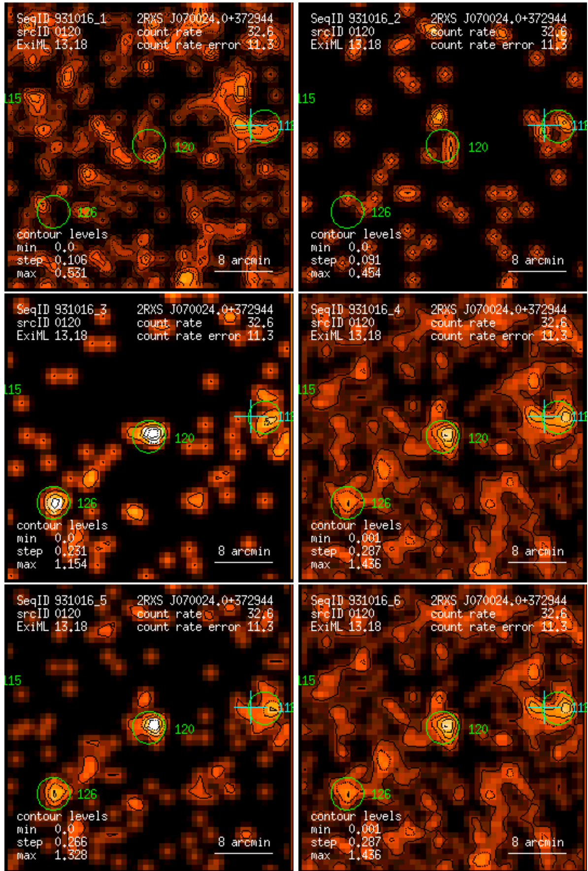
Figure 120: RASS 931016: detection 0120: band rate images, Gaussian filter: (1) PSPC channels 11 – 41, (2) 52 – 90, (3) 91 – 201, (4) 11 – 235, (5) 52 – 201, (6) 11 – 201. Broad band rates in counts/ks. Band rate contour levels in counts/ks/arcmin 2 .
