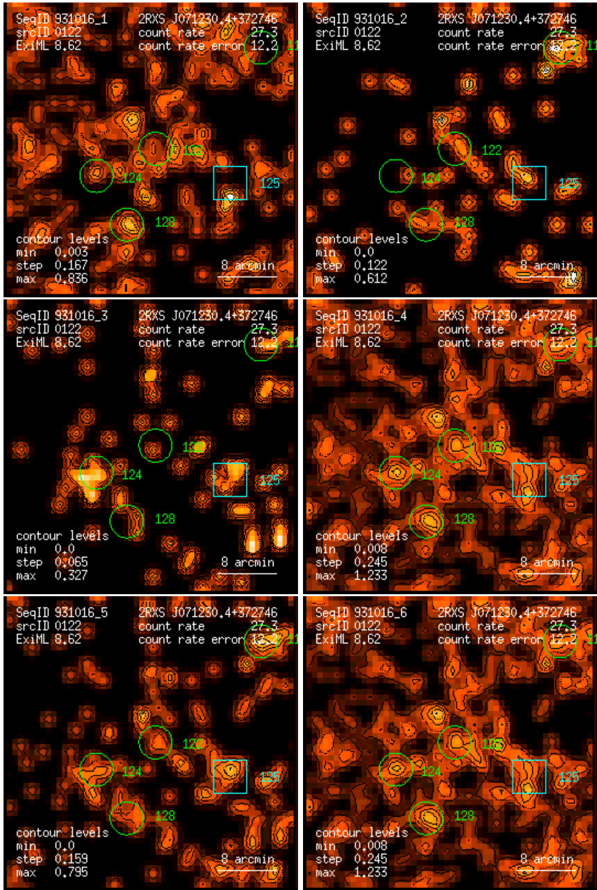
Figure 122: RASS 931016: detection 0122: band rate images, Gaussian filter: (1) PSPC channels 11 – 41, (2) 52 – 90, (3) 91 – 201, (4) 11 – 235, (5) 52 – 201, (6) 11 – 201. Broad band rates in counts/ks. Band rate contour levels in counts/ks/arcmin 2 .
