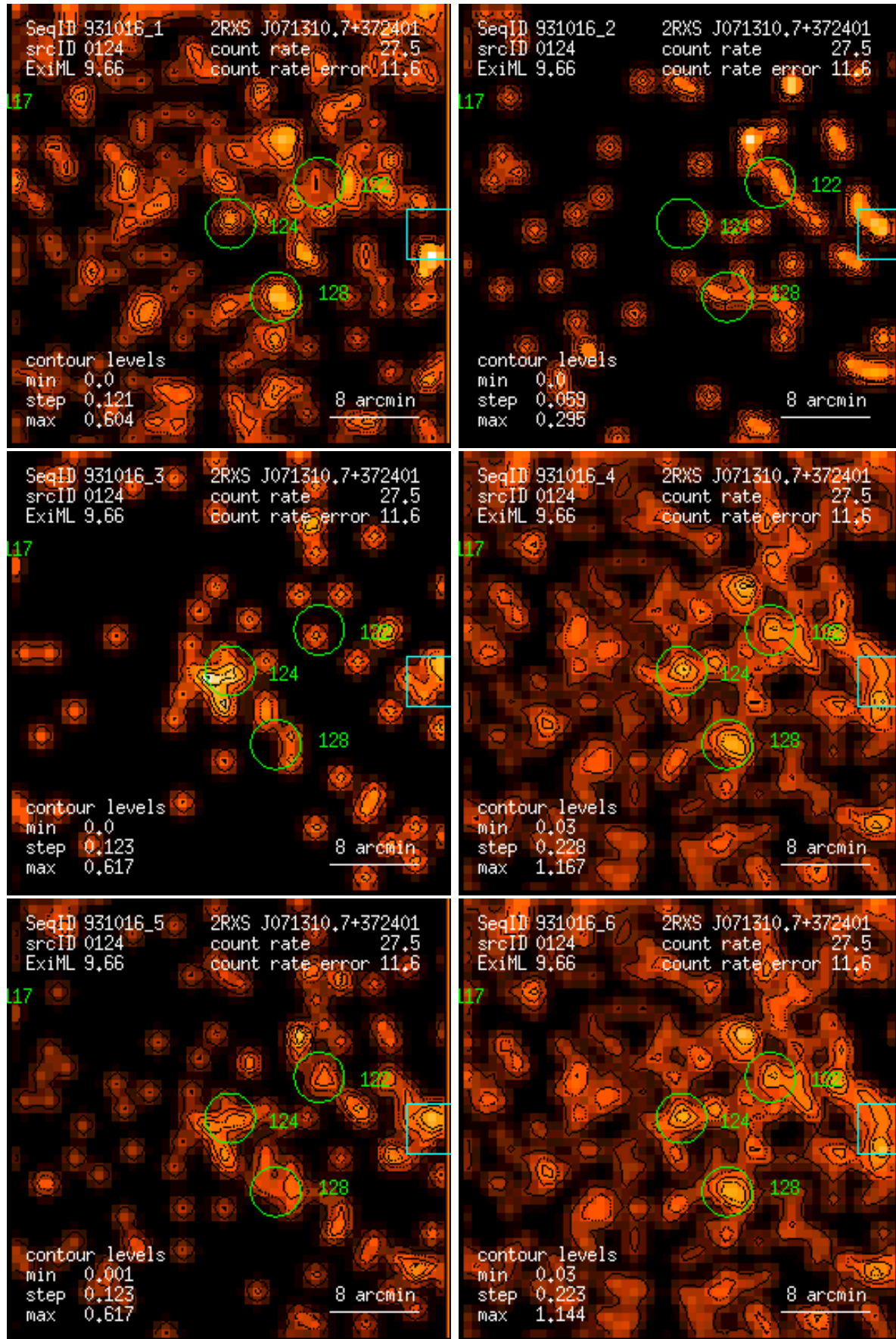
Figure 124: RASS 931016: detection 0124: band rate images, Gaussian filter: (1) PSPC channels 11 – 41, (2) 52 – 90, (3) 91 – 201, (4) 11 – 235, (5) 52 – 201, (6) 11 – 201. Broad band rates in counts/ks. Band rate contour levels in counts/ks/arcmin 2 .
