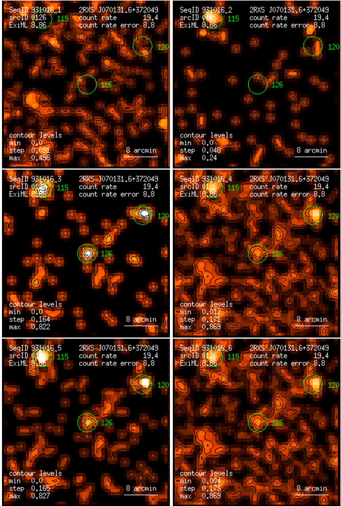
Figure 126: RASS 931016: detection 0126: band rate images, Gaussian filter: (1) PSPC channels 11 – 41, (2) 52 – 90, (3) 91 – 201, (4) 11 – 235, (5) 52 – 201, (6) 11 – 201. Broad band rates in counts/ks. Band rate contour levels in counts/ks/arcmin 2 .
