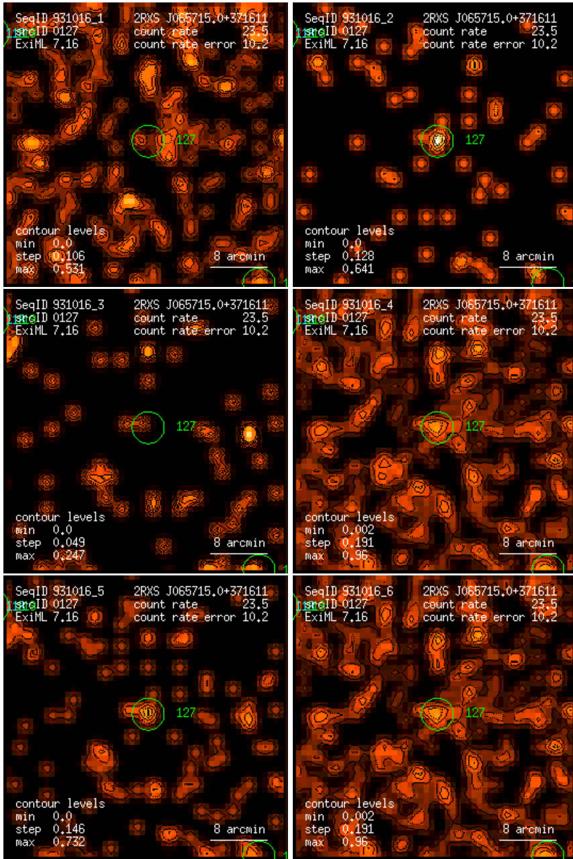
Figure 127: RASS 931016: detection 0127: band rate images, Gaussian filter: (1) PSPC channels 11 – 41, (2) 52 – 90, (3) 91 – 201, (4) 11 – 235, (5) 52 – 201, (6) 11 – 201. Broad band rates in counts/ks. Band rate contour levels in counts/ks/arcmin 2 .
