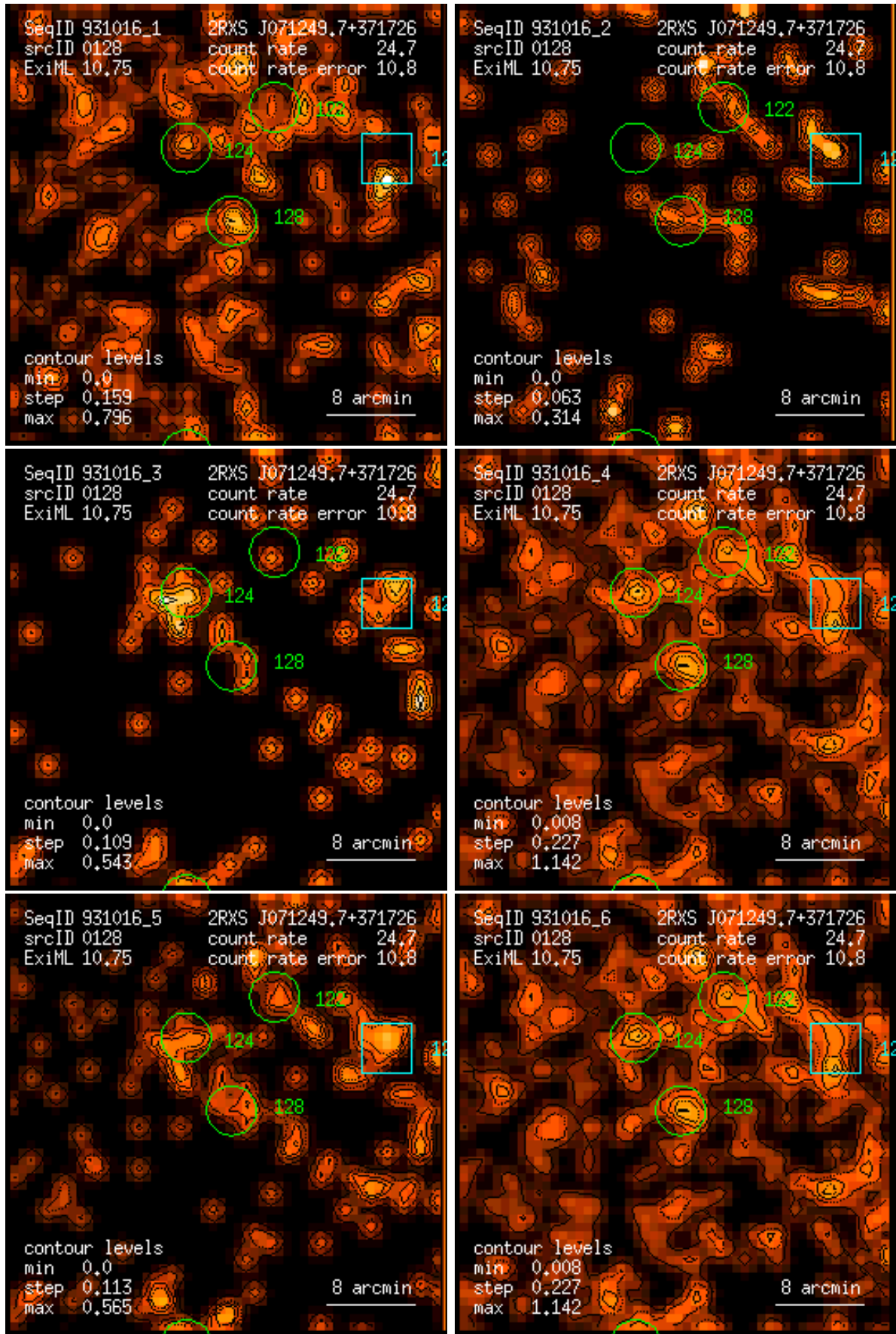
Figure 128: RASS 931016: detection 0128: band rate images, Gaussian filter: (1) PSPC channels 11 – 41, (2) 52 – 90, (3) 91 – 201, (4) 11 – 235, (5) 52 – 201, (6) 11 – 201. Broad band rates in counts/ks. Band rate contour levels in counts/ks/arcmin 2 .
