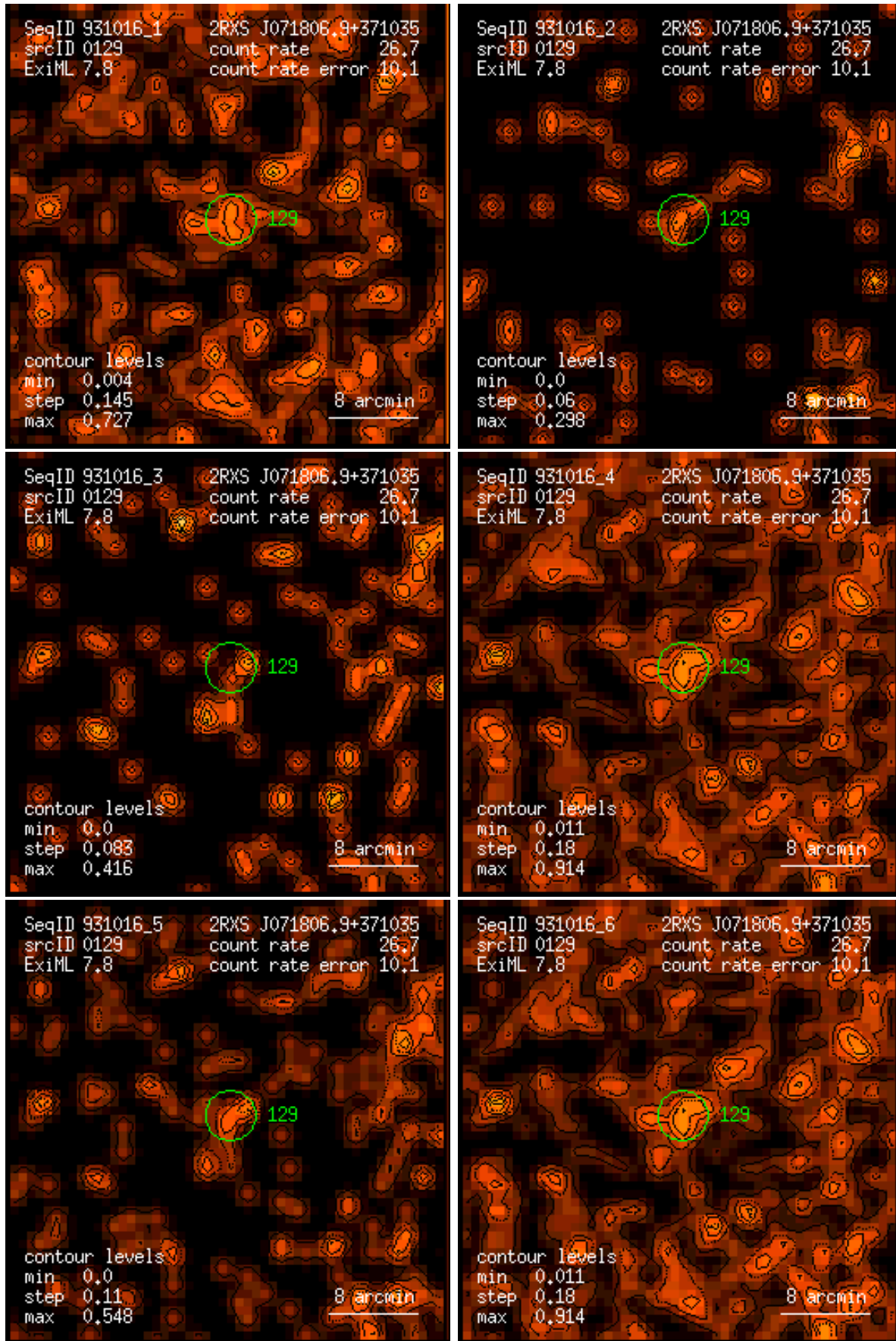
Figure 129: RASS 931016: detection 0129: band rate images, Gaussian filter: (1) PSPC channels 11 – 41, (2) 52 – 90, (3) 91 – 201, (4) 11 – 235, (5) 52 – 201, (6) 11 – 201. Broad band rates in counts/ks. Band rate contour levels in counts/ks/arcmin 2 .
