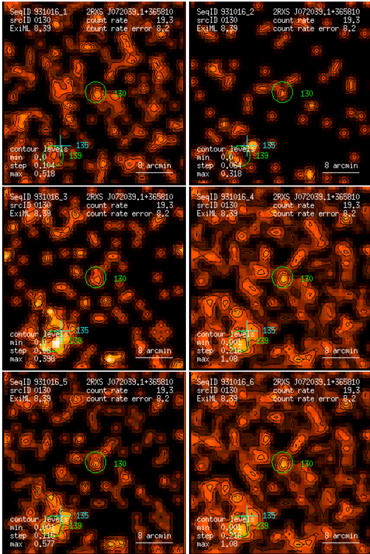
Figure 130: RASS 931016: detection 0130: band rate images, Gaussian filter: (1) PSPC channels 11 – 41, (2) 52 – 90, (3) 91 – 201, (4) 11 – 235, (5) 52 – 201, (6) 11 – 201. Broad band rates in counts/ks. Band rate contour levels in counts/ks/arcmin 2 .
