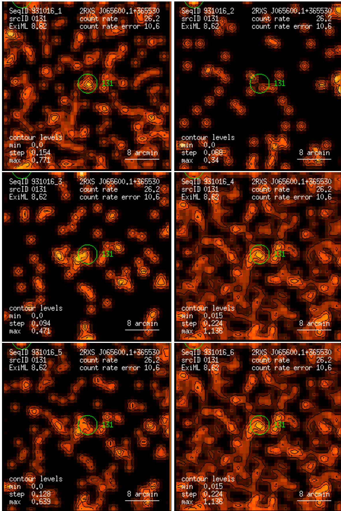
Figure 131: RASS 931016: detection 0131: band rate images, Gaussian filter: (1) PSPC channels 11 – 41, (2) 52 – 90, (3) 91 – 201, (4) 11 – 235, (5) 52 – 201, (6) 11 – 201. Broad band rates in counts/ks. Band rate contour levels in counts/ks/arcmin 2 .
