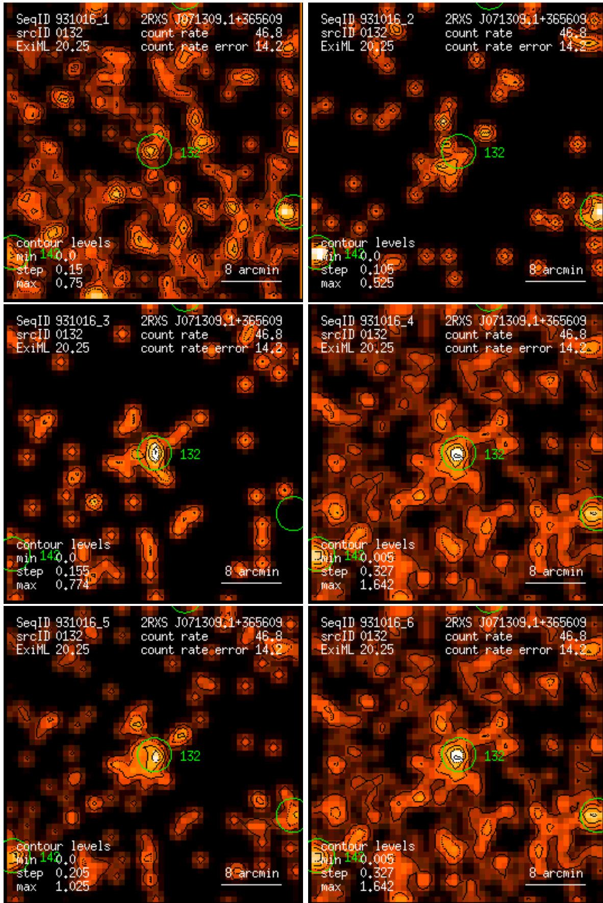
Figure 132: RASS 931016: detection 0132: band rate images, Gaussian filter: (1) PSPC channels 11 – 41, (2) 52 – 90, (3) 91 – 201, (4) 11 – 235, (5) 52 – 201, (6) 11 – 201. Broad band rates in counts/ks. Band rate contour levels in counts/ks/arcmin 2 .
