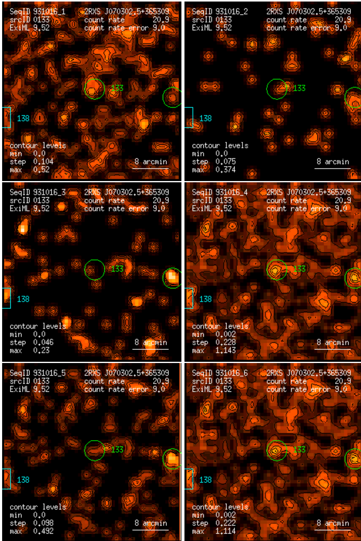
Figure 133: RASS 931016: detection 0133: band rate images, Gaussian filter: (1) PSPC channels 11 – 41, (2) 52 – 90, (3) 91 – 201, (4) 11 – 235, (5) 52 – 201, (6) 11 – 201. Broad band rates in counts/ks. Band rate contour levels in counts/ks/arcmin 2 .
