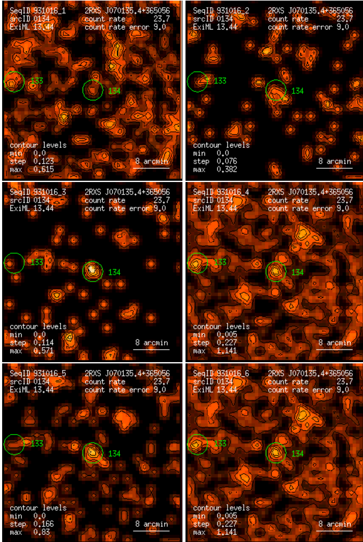
Figure 134: RASS 931016: detection 0134: band rate images, Gaussian filter: (1) PSPC channels 11 – 41, (2) 52 – 90, (3) 91 – 201, (4) 11 – 235, (5) 52 – 201, (6) 11 – 201. Broad band rates in counts/ks. Band rate contour levels in counts/ks/arcmin 2 .
