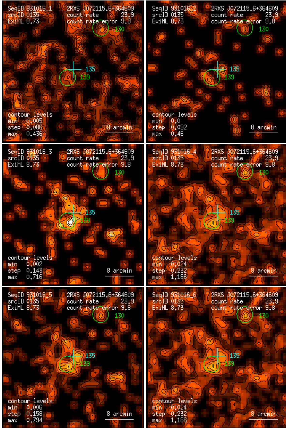
Figure 135: RASS 931016: detection 0135: band rate images, Gaussian filter: (1) PSPC channels 11 – 41, (2) 52 – 90, (3) 91 – 201, (4) 11 – 235, (5) 52 – 201, (6) 11 – 201. Broad band rates in counts/ks. Band rate contour levels in counts/ks/arcmin 2 .
