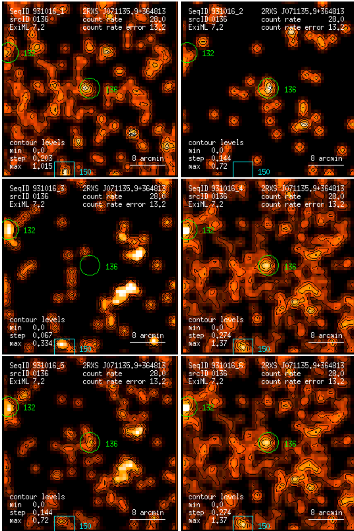
Figure 136: RASS 931016: detection 0136: band rate images, Gaussian filter: (1) PSPC channels 11 – 41, (2) 52 – 90, (3) 91 – 201, (4) 11 – 235, (5) 52 – 201, (6) 11 – 201. Broad band rates in counts/ks. Band rate contour levels in counts/ks/arcmin 2 .
