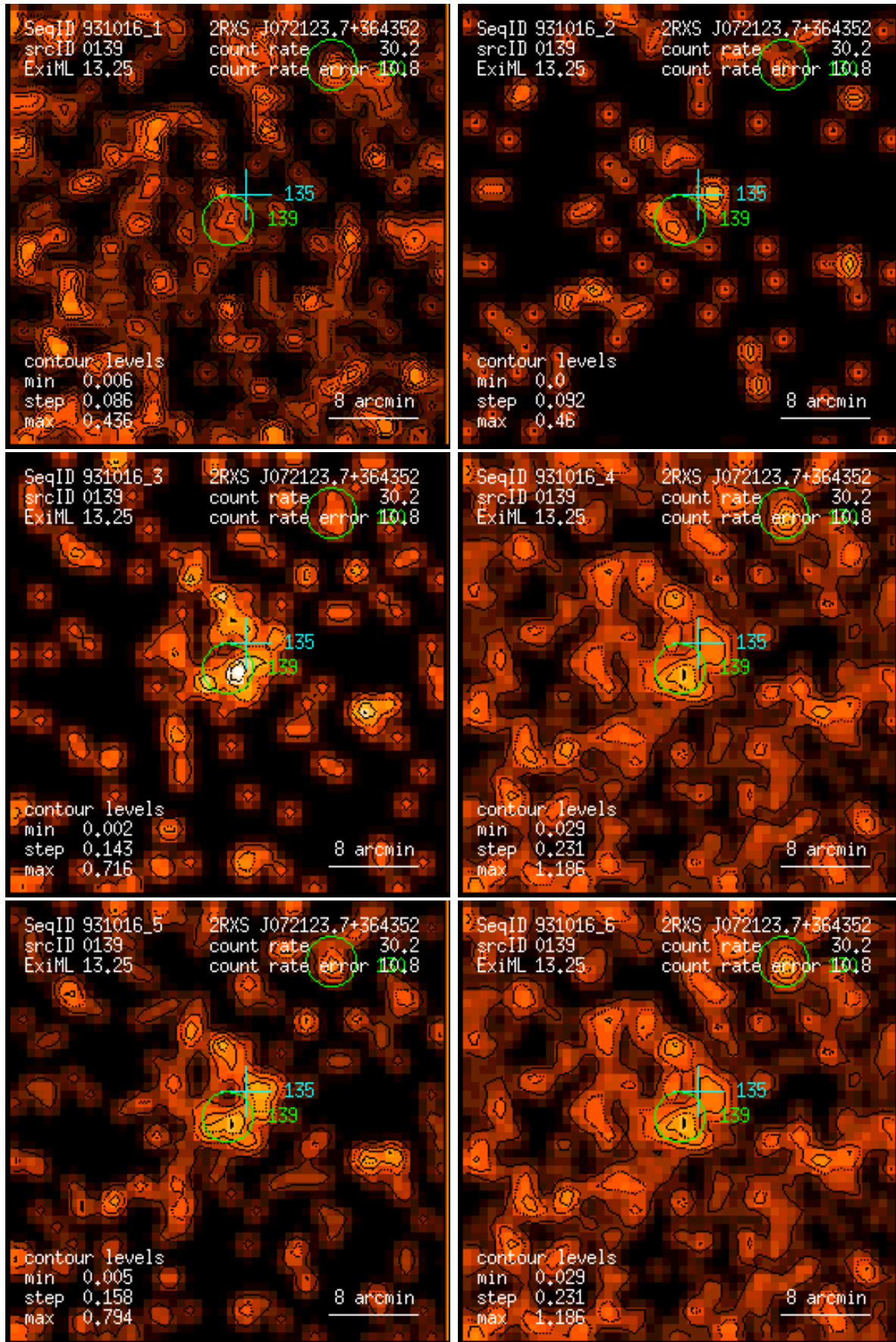
Figure 139: RASS 931016: detection 0139: band rate images, Gaussian filter: (1) PSPC channels 11 – 41, (2) 52 – 90, (3) 91 – 201, (4) 11 – 235, (5) 52 – 201, (6) 11 – 201. Broad band rates in counts/ks. Band rate contour levels in counts/ks/arcmin 2 .
