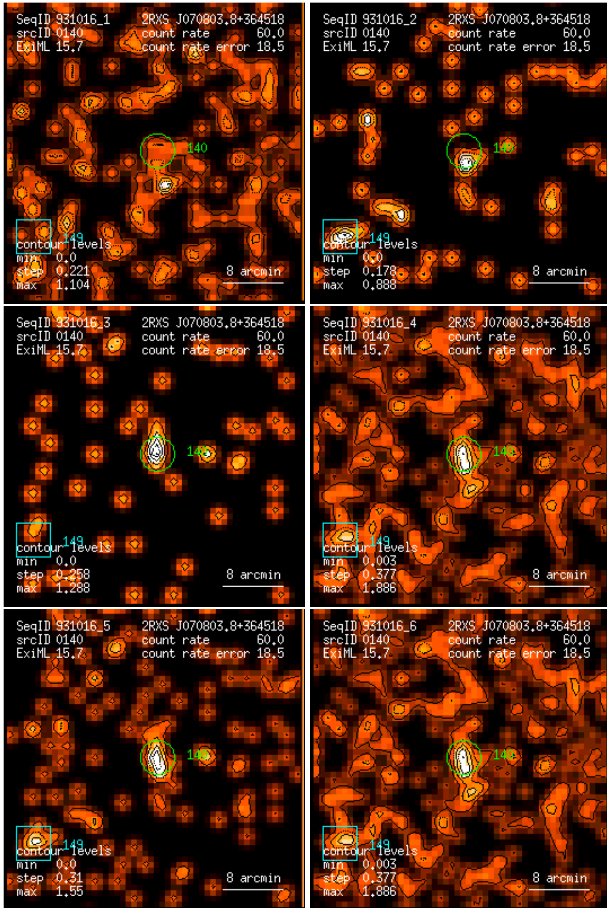
Figure 140: RASS 931016: detection 0140: band rate images, Gaussian filter: (1) PSPC channels 11 – 41, (2) 52 – 90, (3) 91 – 201, (4) 11 – 235, (5) 52 – 201, (6) 11 – 201. Broad band rates in counts/ks. Band rate contour levels in counts/ks/arcmin 2 .
