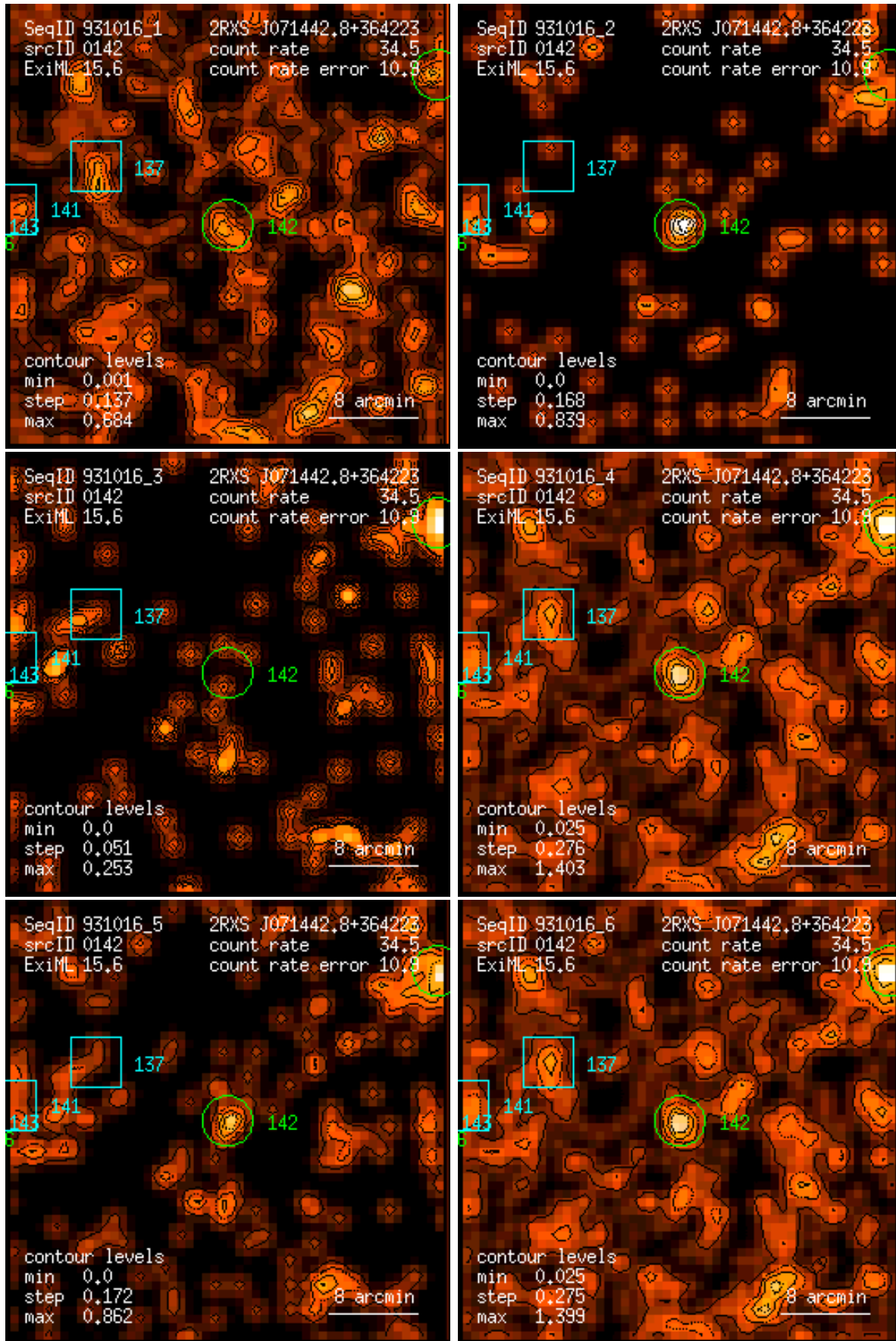
Figure 142: RASS 931016: detection 0142: band rate images, Gaussian filter: (1) PSPC channels 11 – 41, (2) 52 – 90, (3) 91 – 201, (4) 11 – 235, (5) 52 – 201, (6) 11 – 201. Broad band rates in counts/ks. Band rate contour levels in counts/ks/arcmin 2 .
