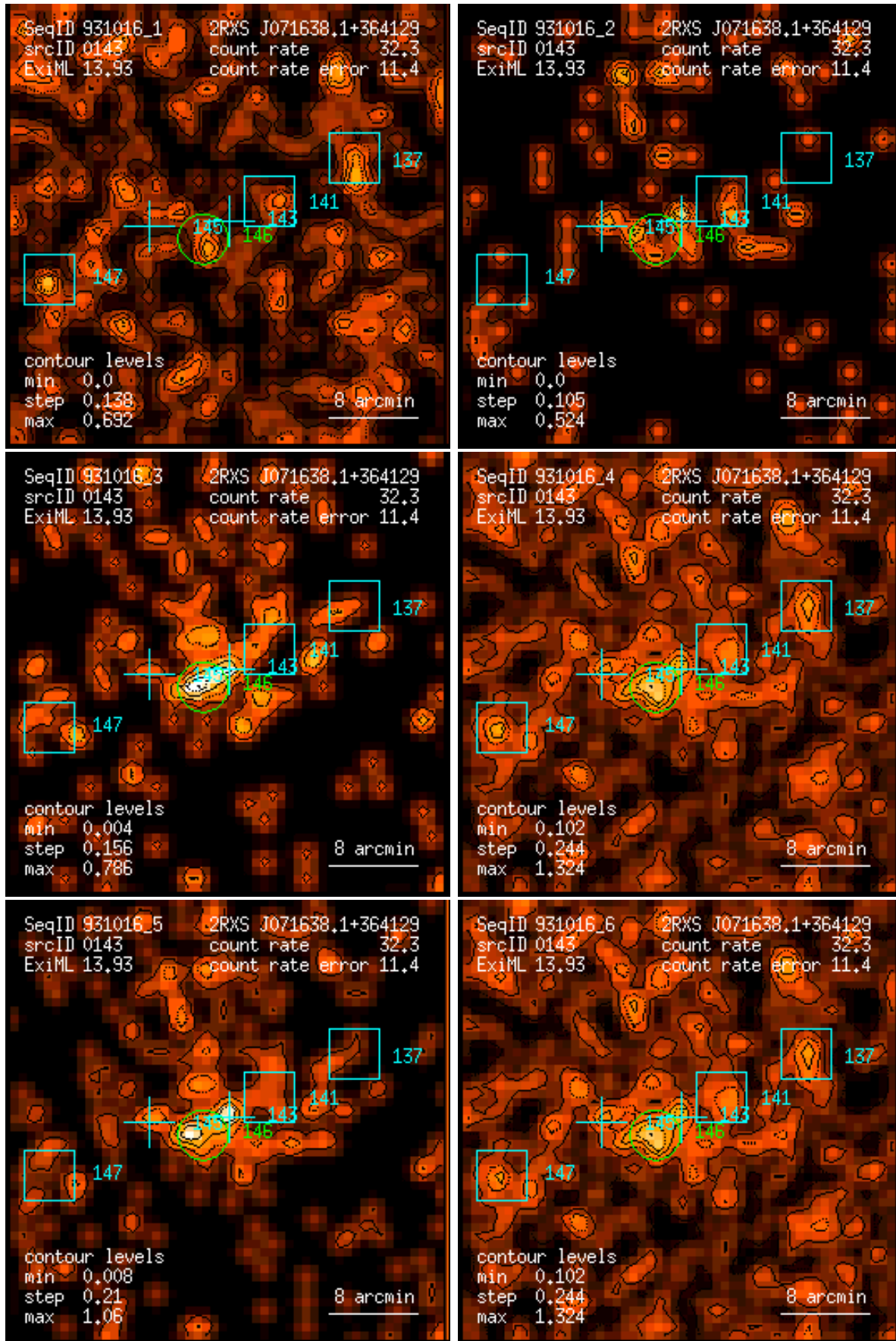
Figure 143: RASS 931016: detection 0143: band rate images, Gaussian filter: (1) PSPC channels 11 – 41, (2) 52 – 90, (3) 91 – 201, (4) 11 – 235, (5) 52 – 201, (6) 11 – 201. Broad band rates in counts/ks. Band rate contour levels in counts/ks/arcmin 2 .
