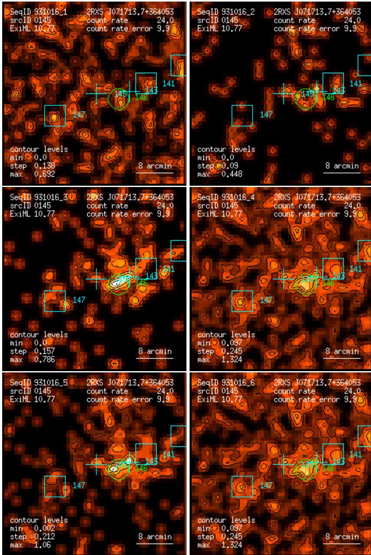
Figure 145: RASS 931016: detection 0145: band rate images, Gaussian filter: (1) PSPC channels 11 – 41, (2) 52 – 90, (3) 91 – 201, (4) 11 – 235, (5) 52 – 201, (6) 11 – 201. Broad band rates in counts/ks. Band rate contour levels in counts/ks/arcmin 2 .
