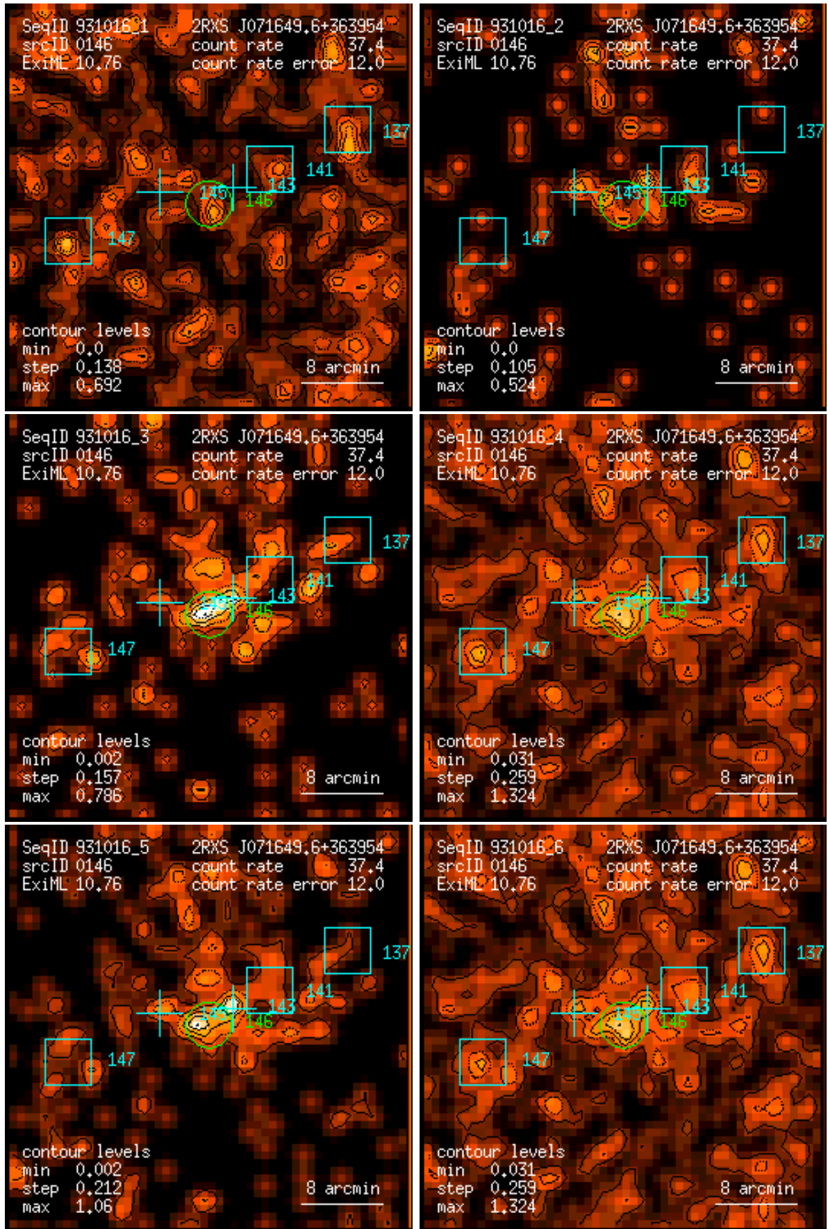
Figure 146: RASS 931016: detection 0146: band rate images, Gaussian filter: (1) PSPC channels 11 – 41, (2) 52 – 90, (3) 91 – 201, (4) 11 – 235, (5) 52 – 201, (6) 11 – 201. Broad band rates in counts/ks. Band rate contour levels in counts/ks/arcmin 2 .
