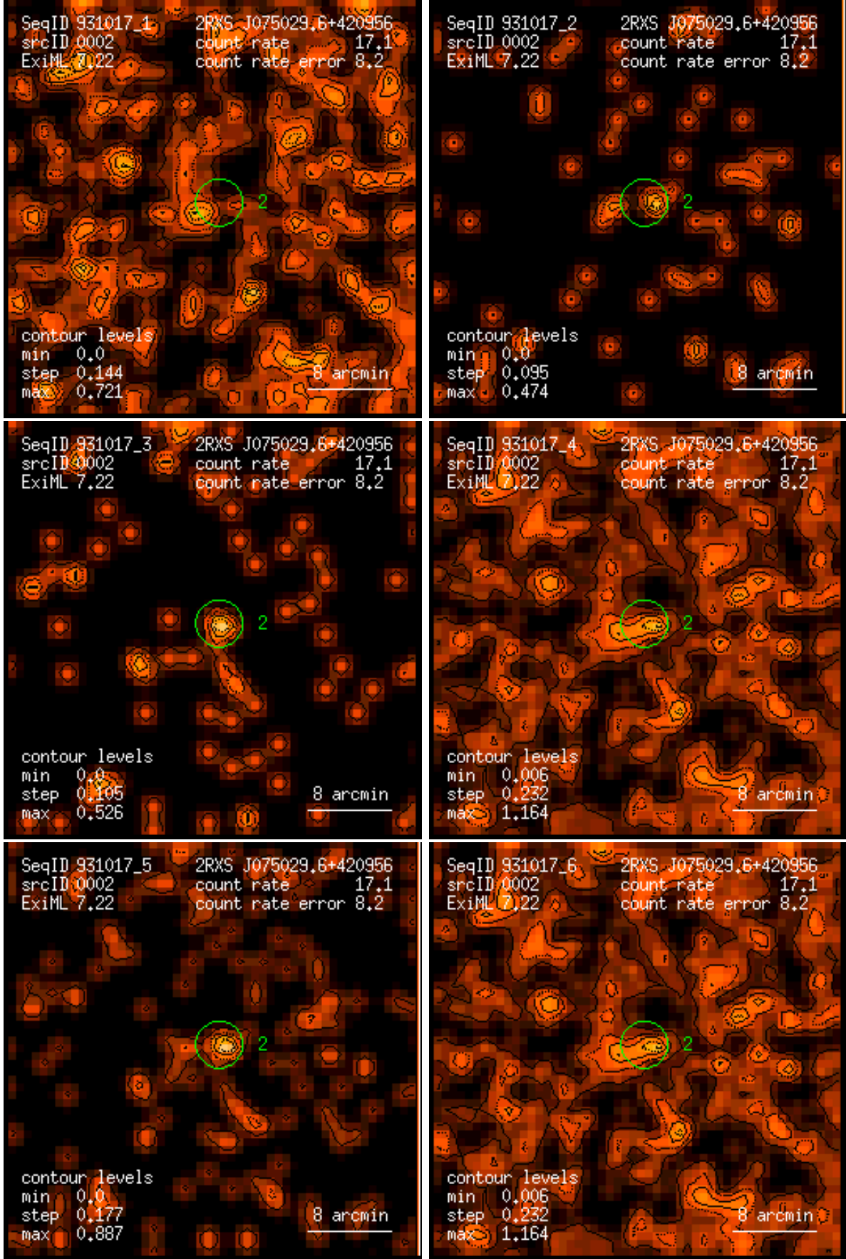
Figure 2: RASS 931017: detection 0002: band rate images, Gaussian filter: (1) PSPC channels 11 – 41, (2) 52 – 90, (3) 91 – 201, (4) 11 – 235, (5) 52 – 201, (6) 11 – 201. Broad band rates in counts/ks. Band rate contour levels in counts/ks/arcmin 2 .
