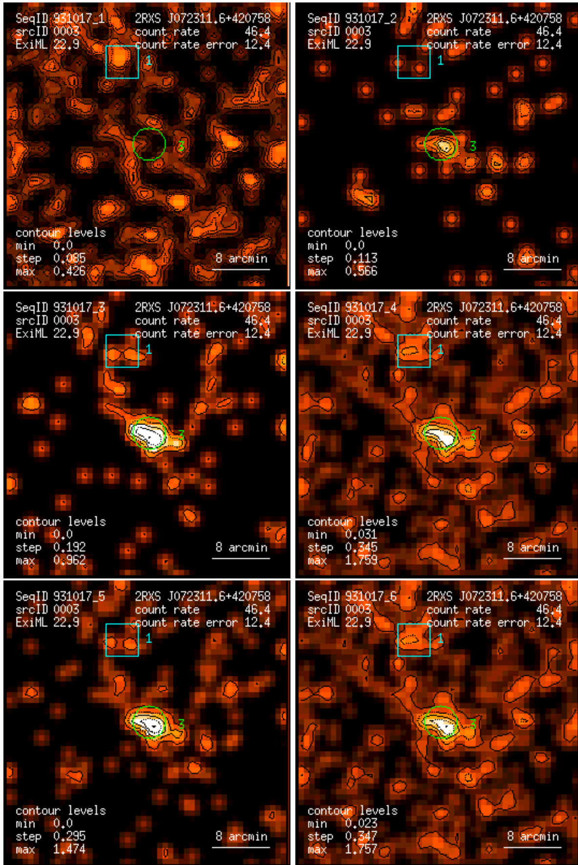
Figure 3: RASS 931017: detection 0003: band rate images, Gaussian filter: (1) PSPC channels 11 – 41, (2) 52 – 90, (3) 91 – 201, (4) 11 – 235, (5) 52 – 201, (6) 11 – 201. Broad band rates in counts/ks. Band rate contour levels in counts/ks/arcmin 2 .
