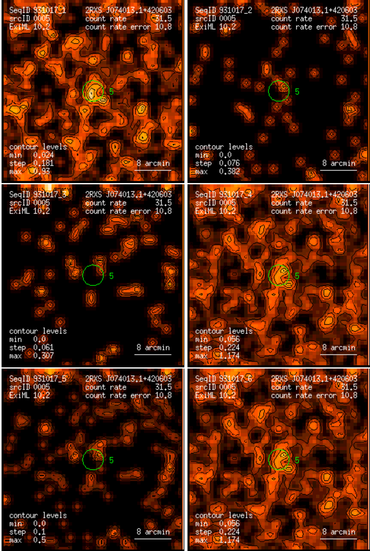
Figure 5: RASS 931017: detection 0005: band rate images, Gaussian filter: (1) PSPC channels 11 – 41, (2) 52 – 90, (3) 91 – 201, (4) 11 – 235, (5) 52 – 201, (6) 11 – 201. Broad band rates in counts/ks. Band rate contour levels in counts/ks/arcmin 2 .
