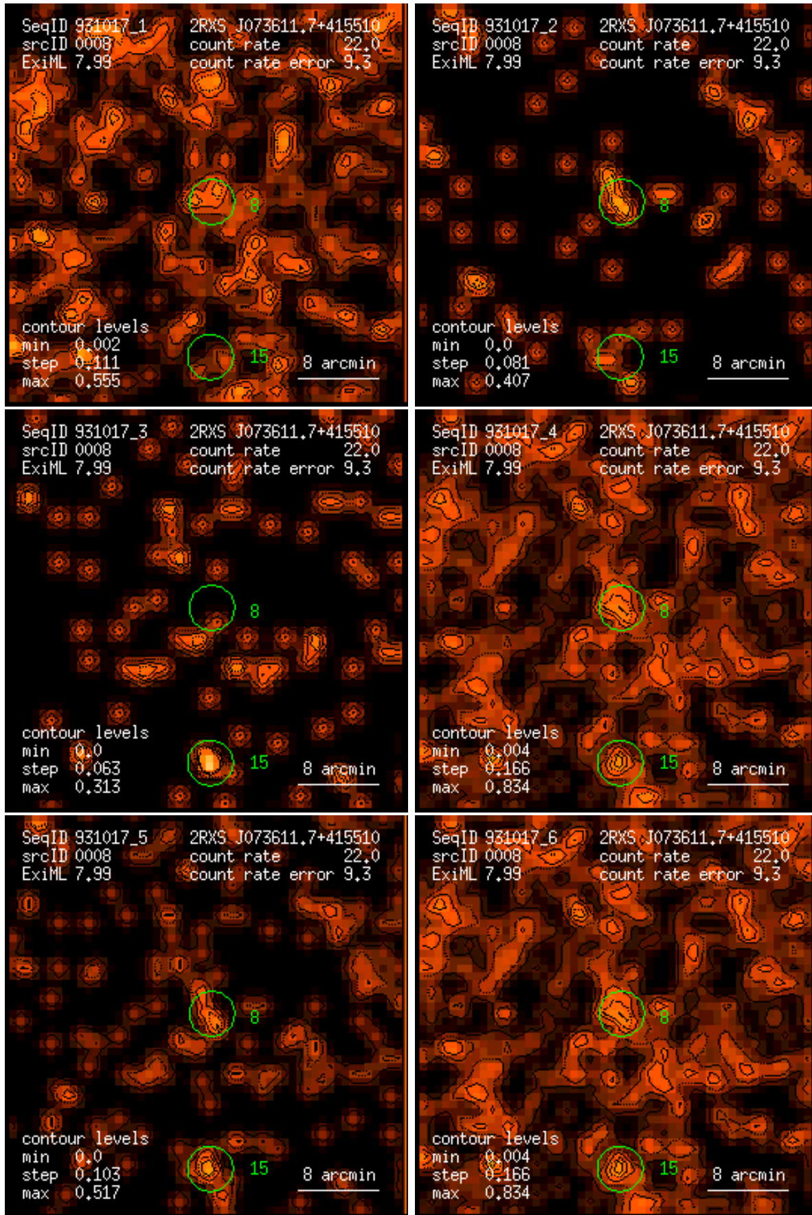
Figure 8: RASS 931017: detection 0008: band rate images, Gaussian filter: (1) PSPC channels 11 – 41, (2) 52 – 90, (3) 91 – 201, (4) 11 – 235, (5) 52 – 201, (6) 11 – 201. Broad band rates in counts/ks. Band rate contour levels in counts/ks/arcmin 2 .
