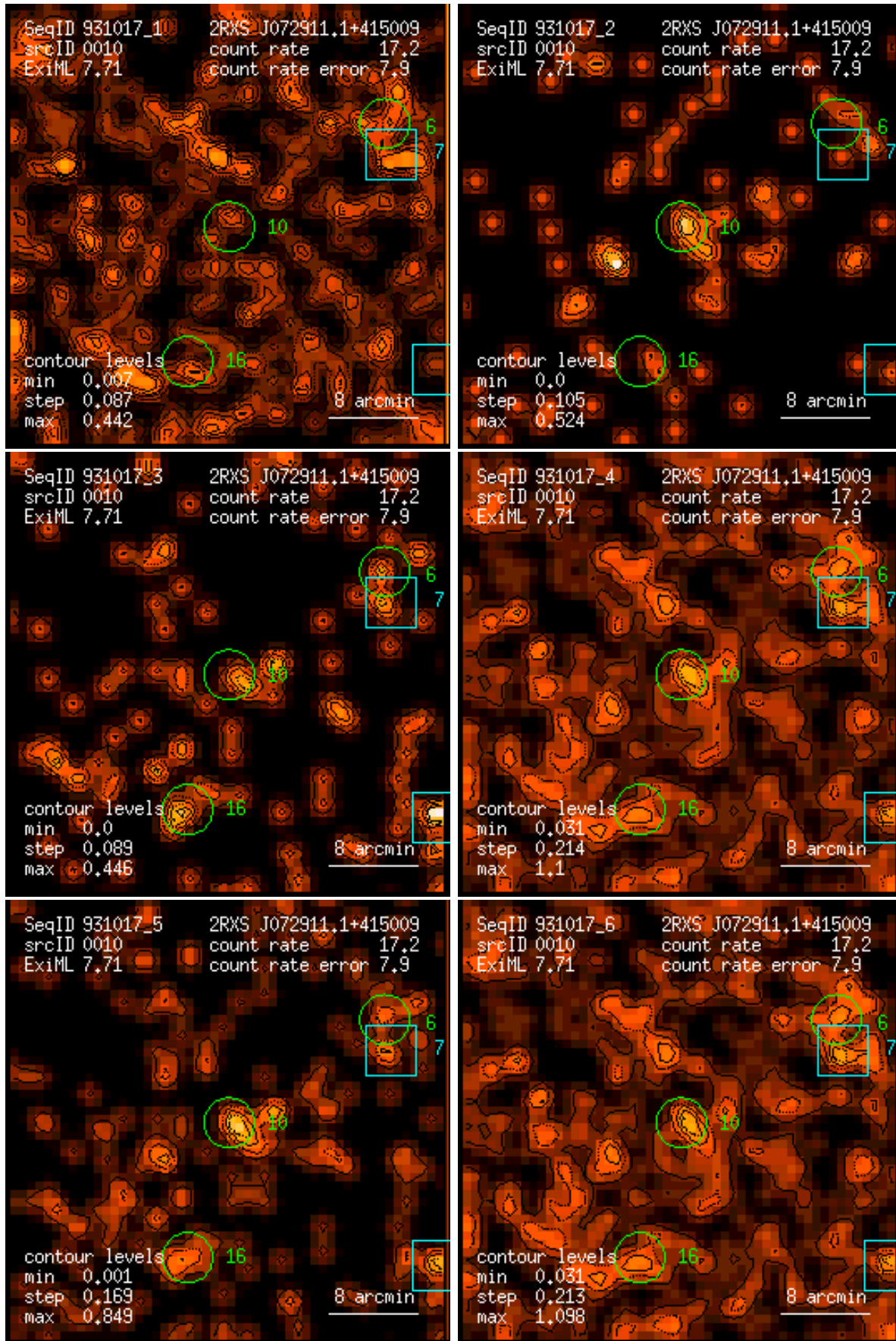
Figure 10: RASS 931017: detection 0010: band rate images, Gaussian filter: (1) PSPC channels 11 – 41, (2) 52 – 90, (3) 91 – 201, (4) 11 – 235, (5) 52 – 201, (6) 11 – 201. Broad band rates in counts/ks. Band rate contour levels in counts/ks/arcmin 2 .
