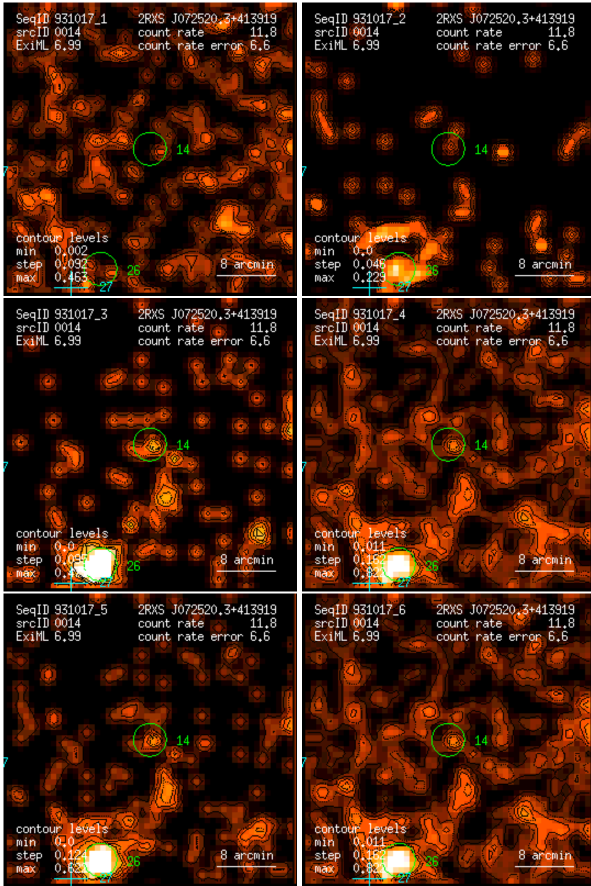
Figure 14: RASS 931017: detection 0014: band rate images, Gaussian filter: (1) PSPC channels 11 – 41, (2) 52 – 90, (3) 91 – 201, (4) 11 – 235, (5) 52 – 201, (6) 11 – 201. Broad band rates in counts/ks. Band rate contour levels in counts/ks/arcmin 2 .
