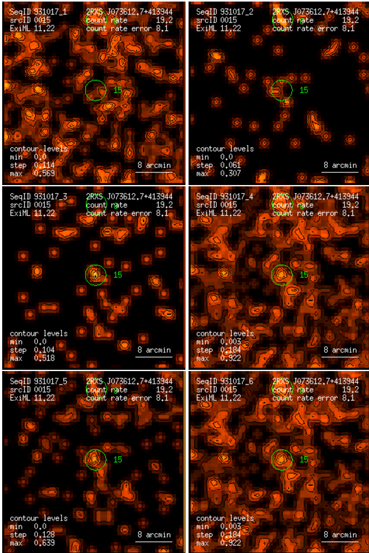
Figure 15: RASS 931017: detection 0015: band rate images, Gaussian filter: (1) PSPC channels 11 – 41, (2) 52 – 90, (3) 91 – 201, (4) 11 – 235, (5) 52 – 201, (6) 11 – 201. Broad band rates in counts/ks. Band rate contour levels in counts/ks/arcmin 2 .
