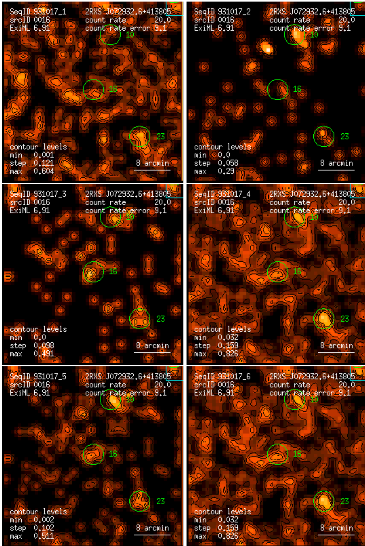
Figure 16: RASS 931017: detection 0016: band rate images, Gaussian filter: (1) PSPC channels 11 – 41, (2) 52 – 90, (3) 91 – 201, (4) 11 – 235, (5) 52 – 201, (6) 11 – 201. Broad band rates in counts/ks. Band rate contour levels in counts/ks/arcmin 2 .
