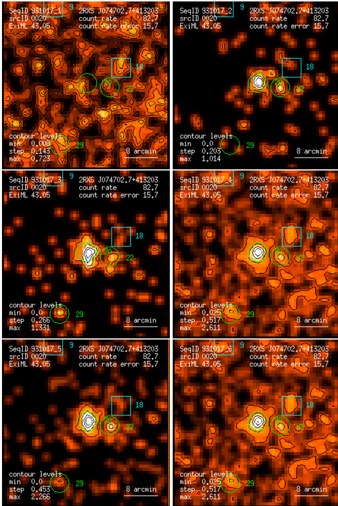
Figure 20: RASS 931017: detection 0020: band rate images, Gaussian filter: (1) PSPC channels 11 – 41, (2) 52 – 90, (3) 91 – 201, (4) 11 – 235, (5) 52 – 201, (6) 11 – 201. Broad band rates in counts/ks. Band rate contour levels in counts/ks/arcmin 2 .
