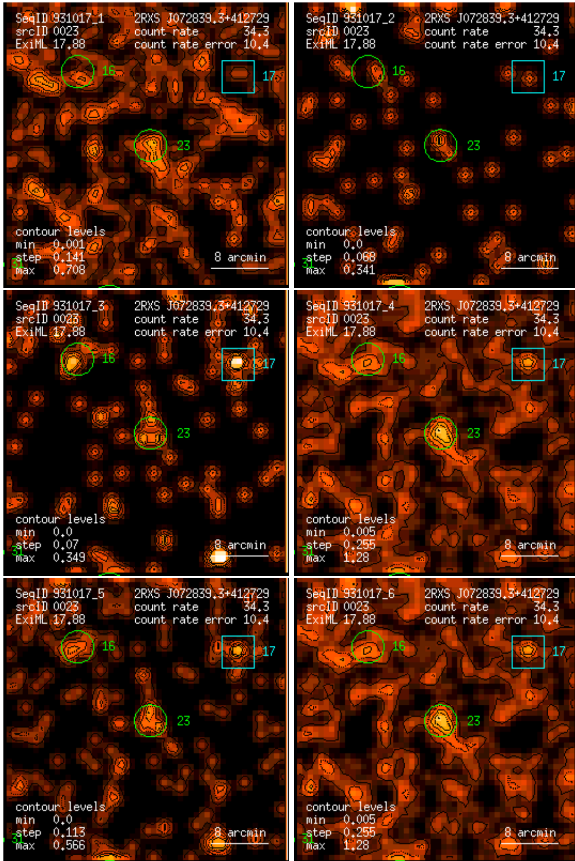
Figure 23: RASS 931017: detection 0023: band rate images, Gaussian filter: (1) PSPC channels 11 – 41, (2) 52 – 90, (3) 91 – 201, (4) 11 – 235, (5) 52 – 201, (6) 11 – 201. Broad band rates in counts/ks. Band rate contour levels in counts/ks/arcmin 2 .
