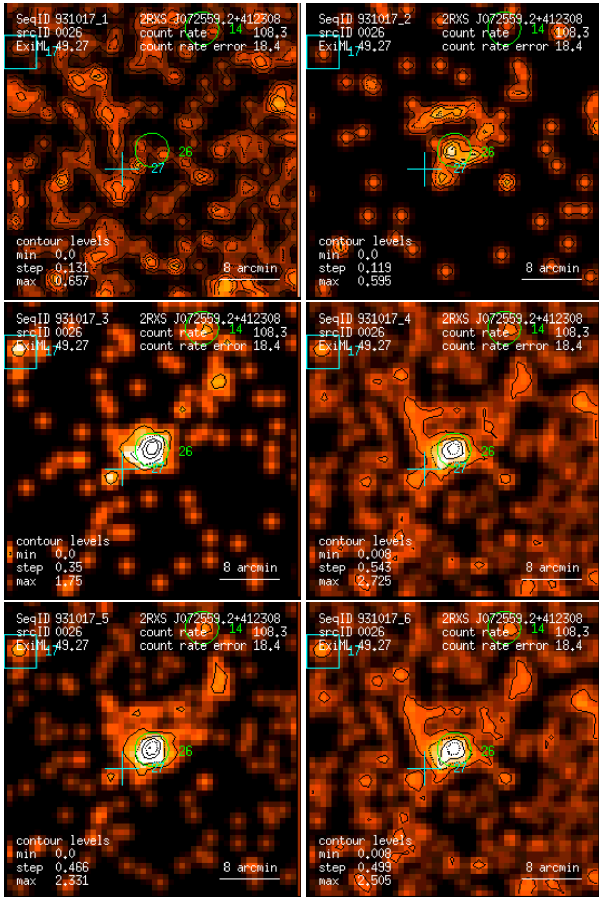
Figure 26: RASS 931017: detection 0026: band rate images, Gaussian filter: (1) PSPC channels 11 – 41, (2) 52 – 90, (3) 91 – 201, (4) 11 – 235, (5) 52 – 201, (6) 11 – 201. Broad band rates in counts/ks. Band rate contour levels in counts/ks/arcmin 2 .
