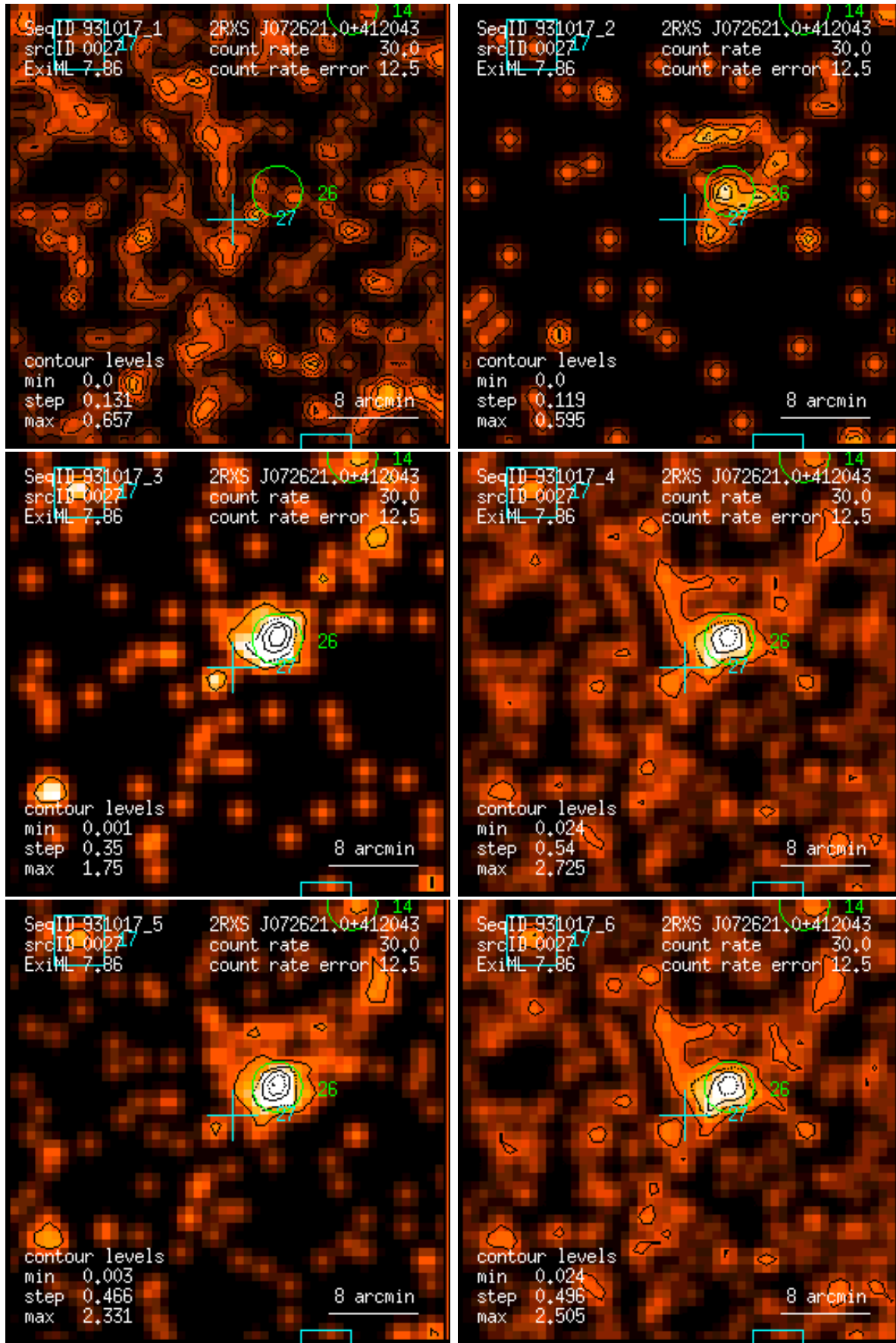
Figure 27: RASS 931017: detection 0027: band rate images, Gaussian filter: (1) PSPC channels 11 – 41, (2) 52 – 90, (3) 91 – 201, (4) 11 – 235, (5) 52 – 201, (6) 11 – 201. Broad band rates in counts/ks. Band rate contour levels in counts/ks/arcmin 2 .
